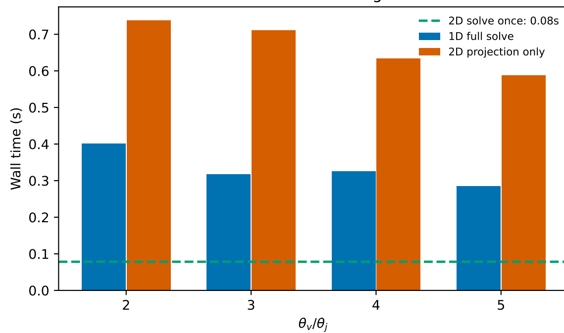
Benchmark timings
