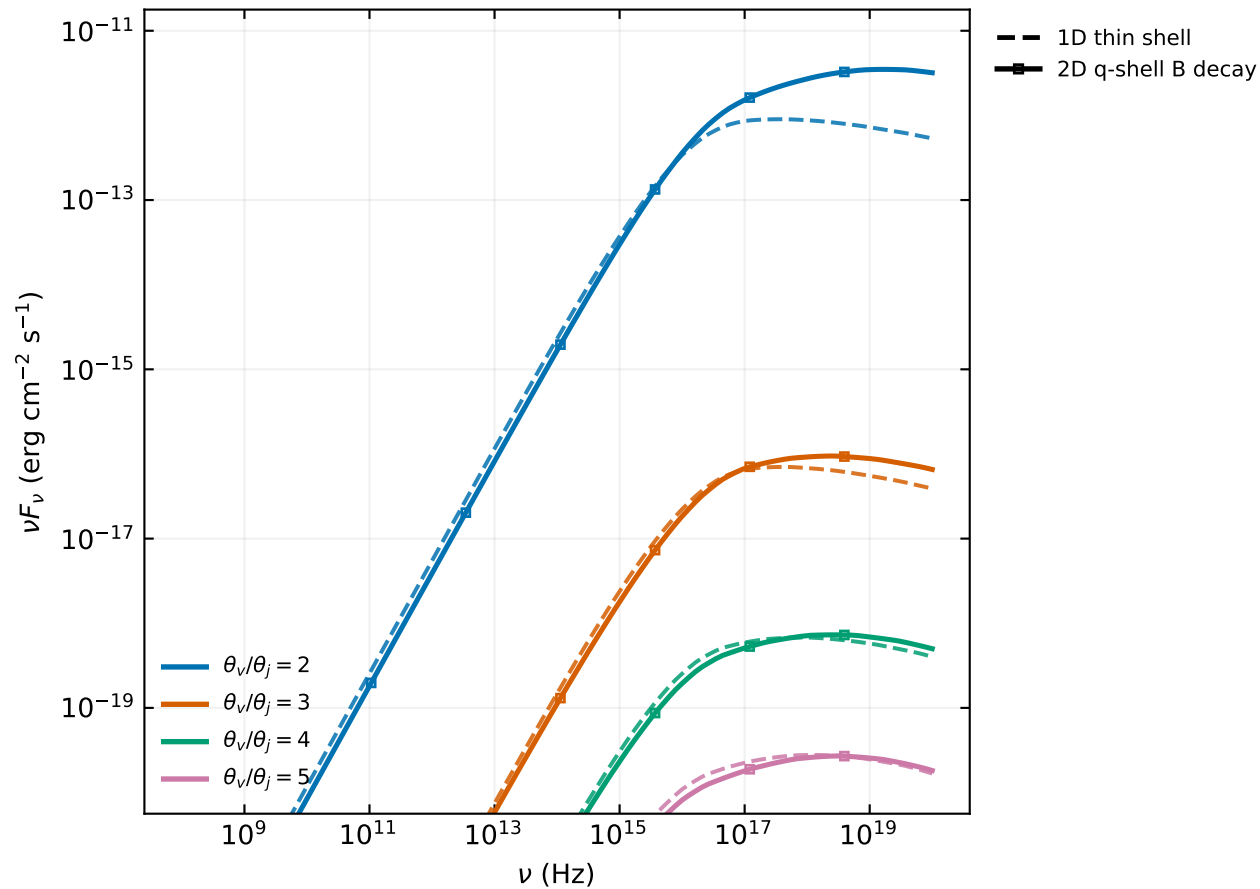
Spectrum at t_{\text{obs}} = 10^4 s
