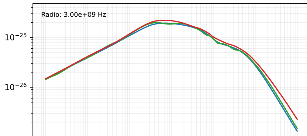
WIND forward-shock + SSC
