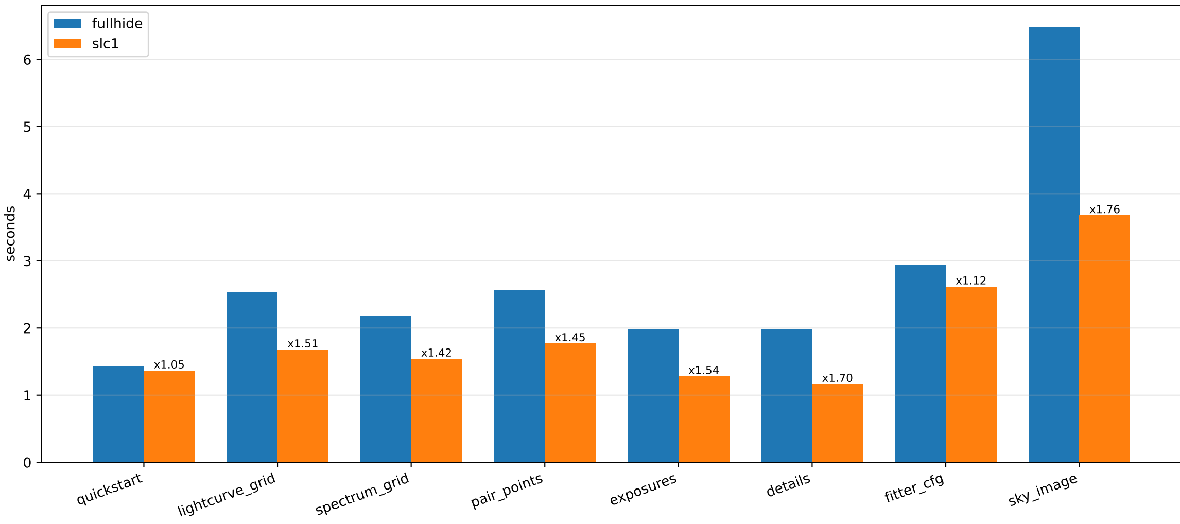
ASGARD README benchmark: fullhide vs slc1
