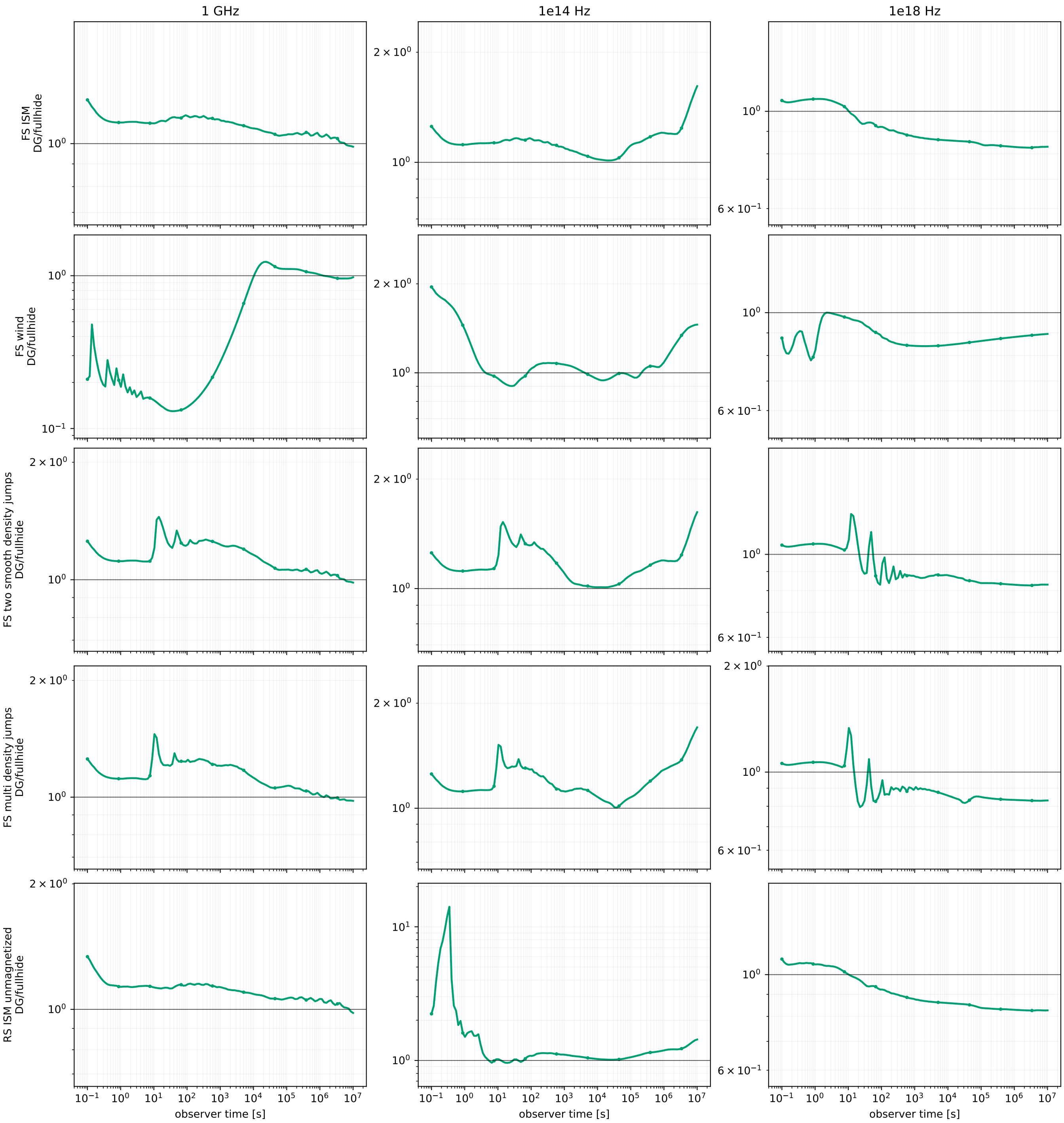
DG1d troubled positive-kernel benchmark: light-curve ratios
