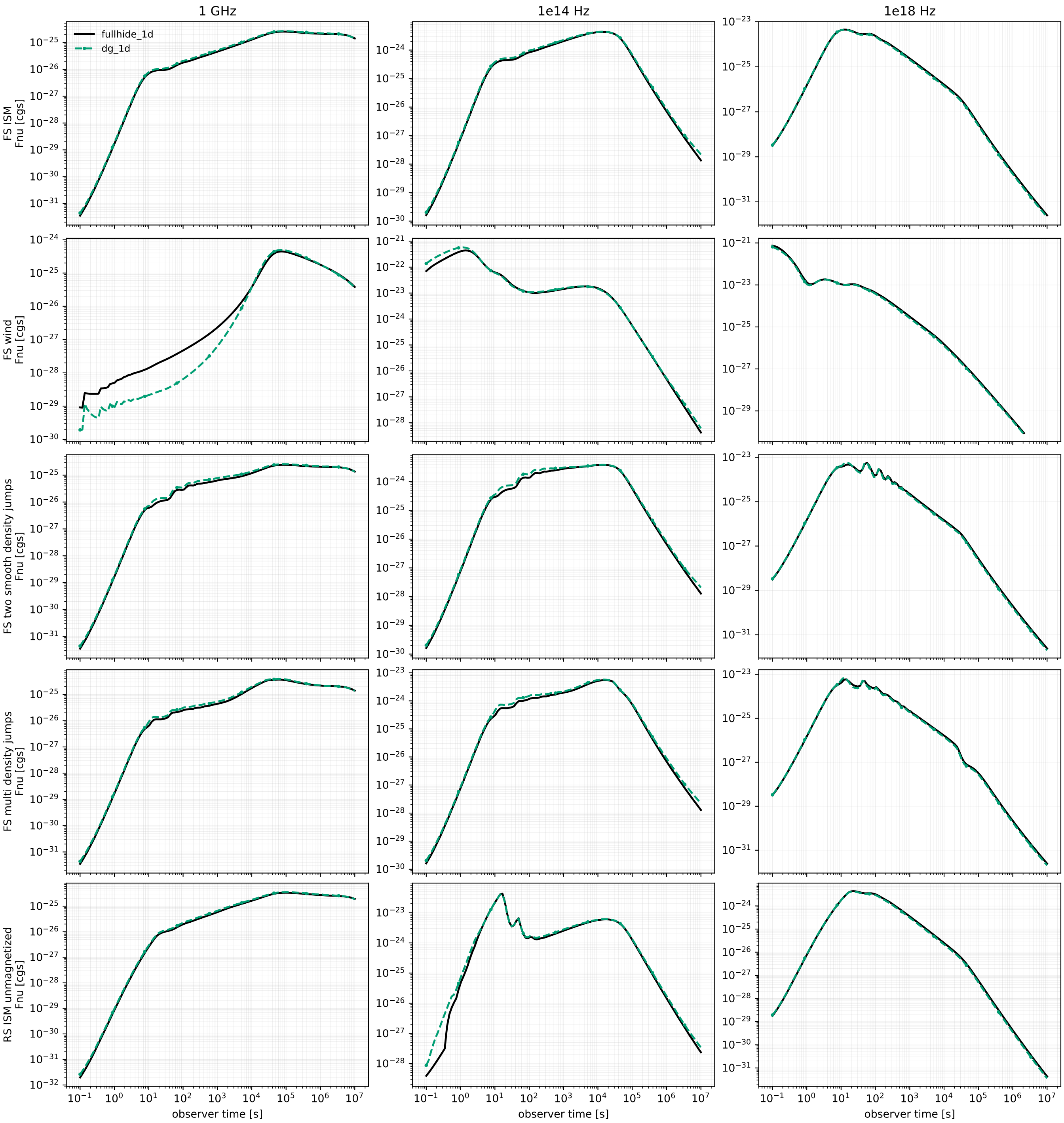
DG1d troubled positive-kernel benchmark: fullhide vs DG total light curves
