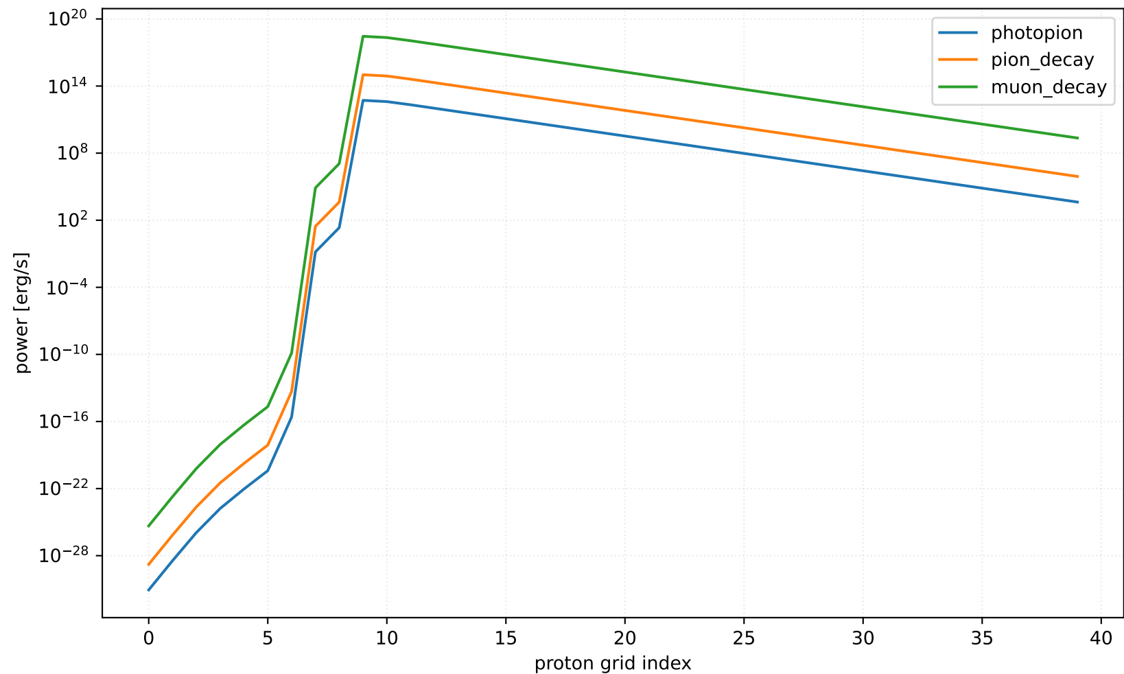
AM3 Process Power Breakdown
