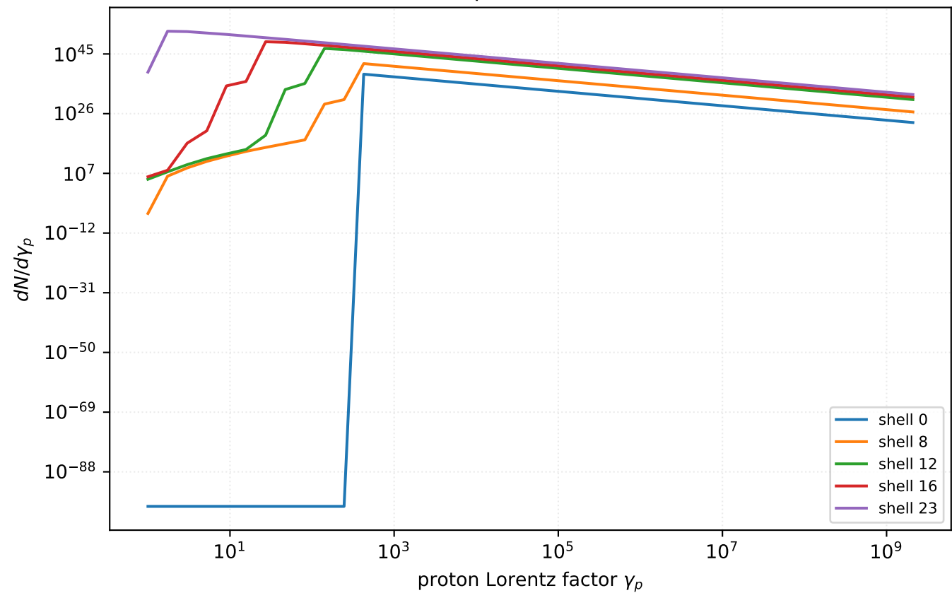
Proton Spectrum Evolution
