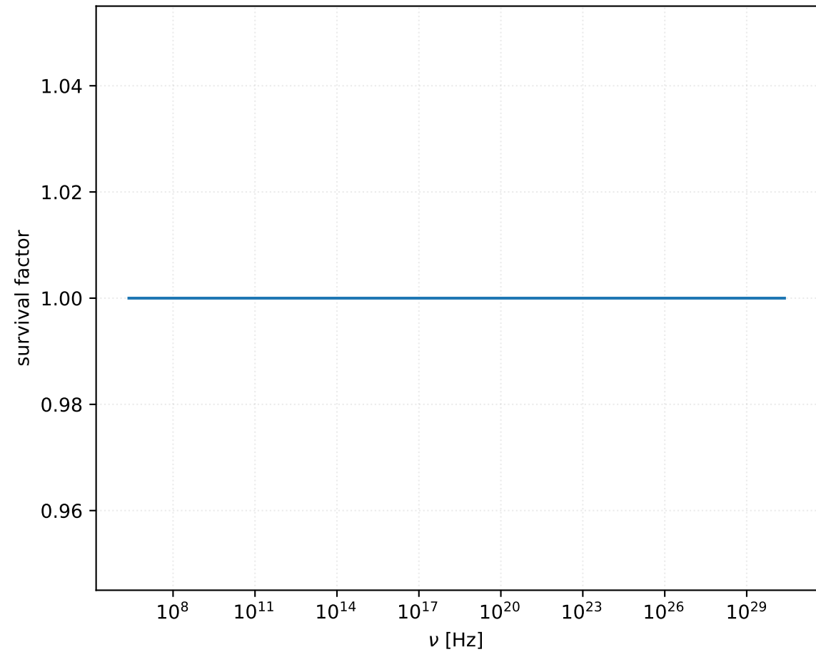
Photon Survival Factor
