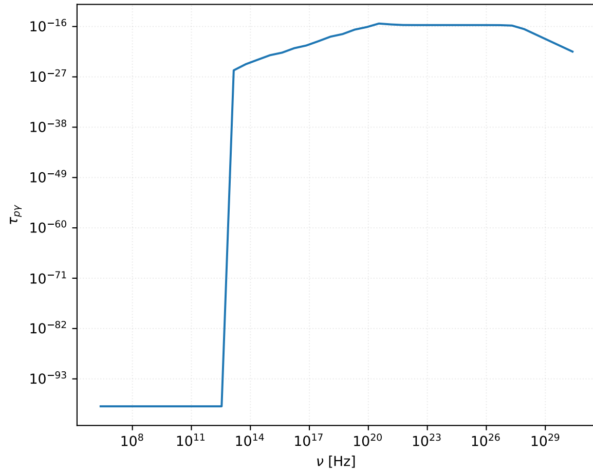
P-Gamma Optical Depth
