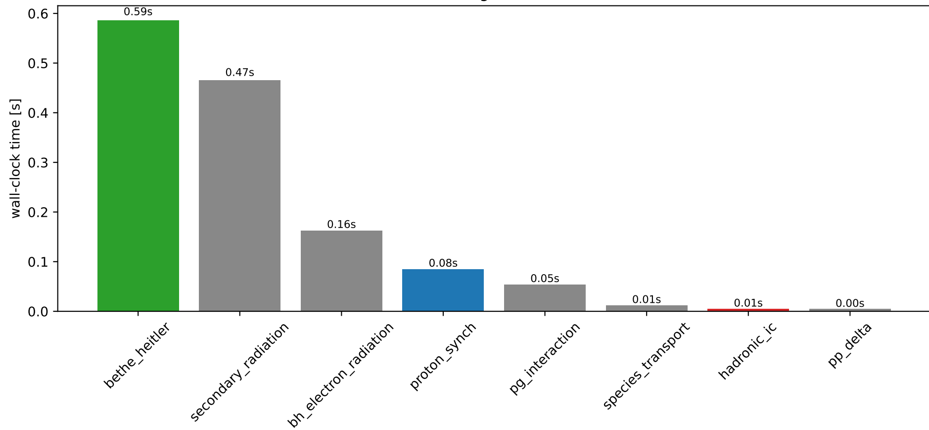
Hadronic Process Timing Breakdown (total=1.40s)
