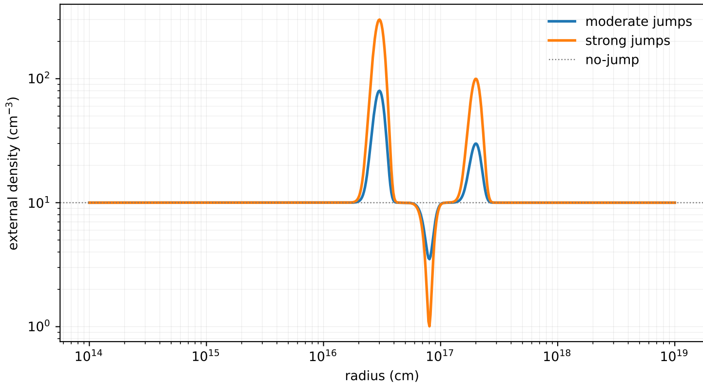
ISM density structures, relative width 0.1
