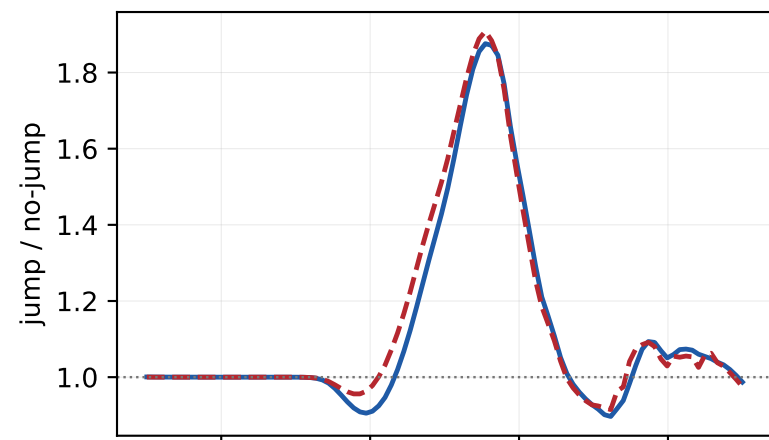
ISM width 0.1 moderate jumps: total-only zoom and jump signal
