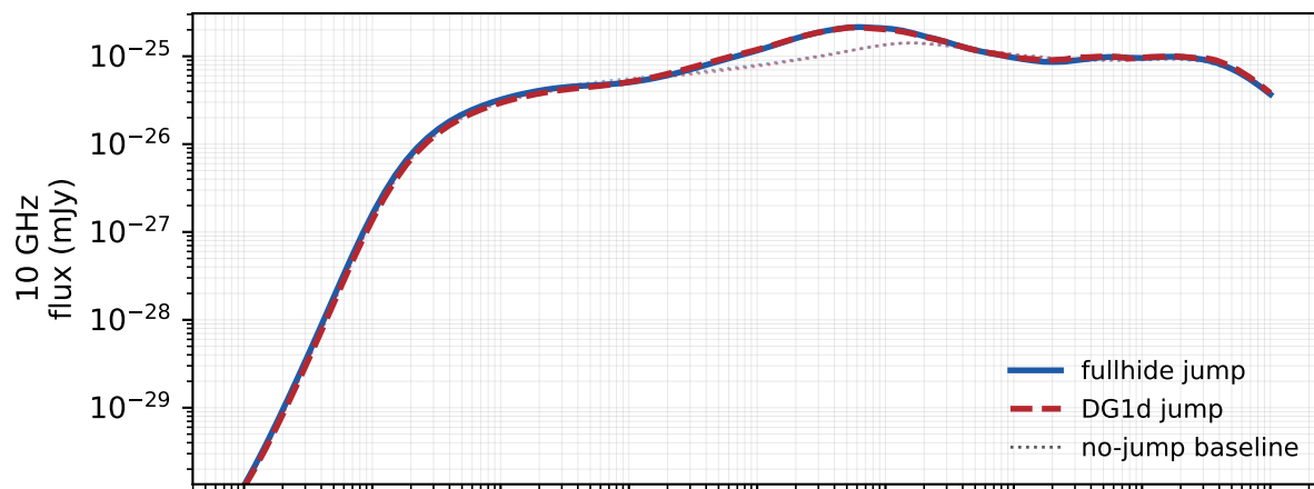
ISM width 0.1 moderate jumps: total-only zoom and jump signal
