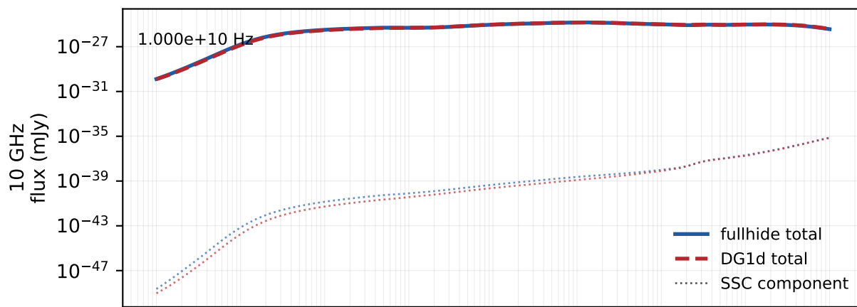
ISM continuous density jumps: strong IC dense FS, eps_e=0.3, eps_B=1e-3, n scaled x10
