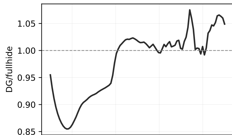
ISM continuous density jumps: strong IC dense FS, eps_e=0.3, eps_B=1e-3, n scaled x10
