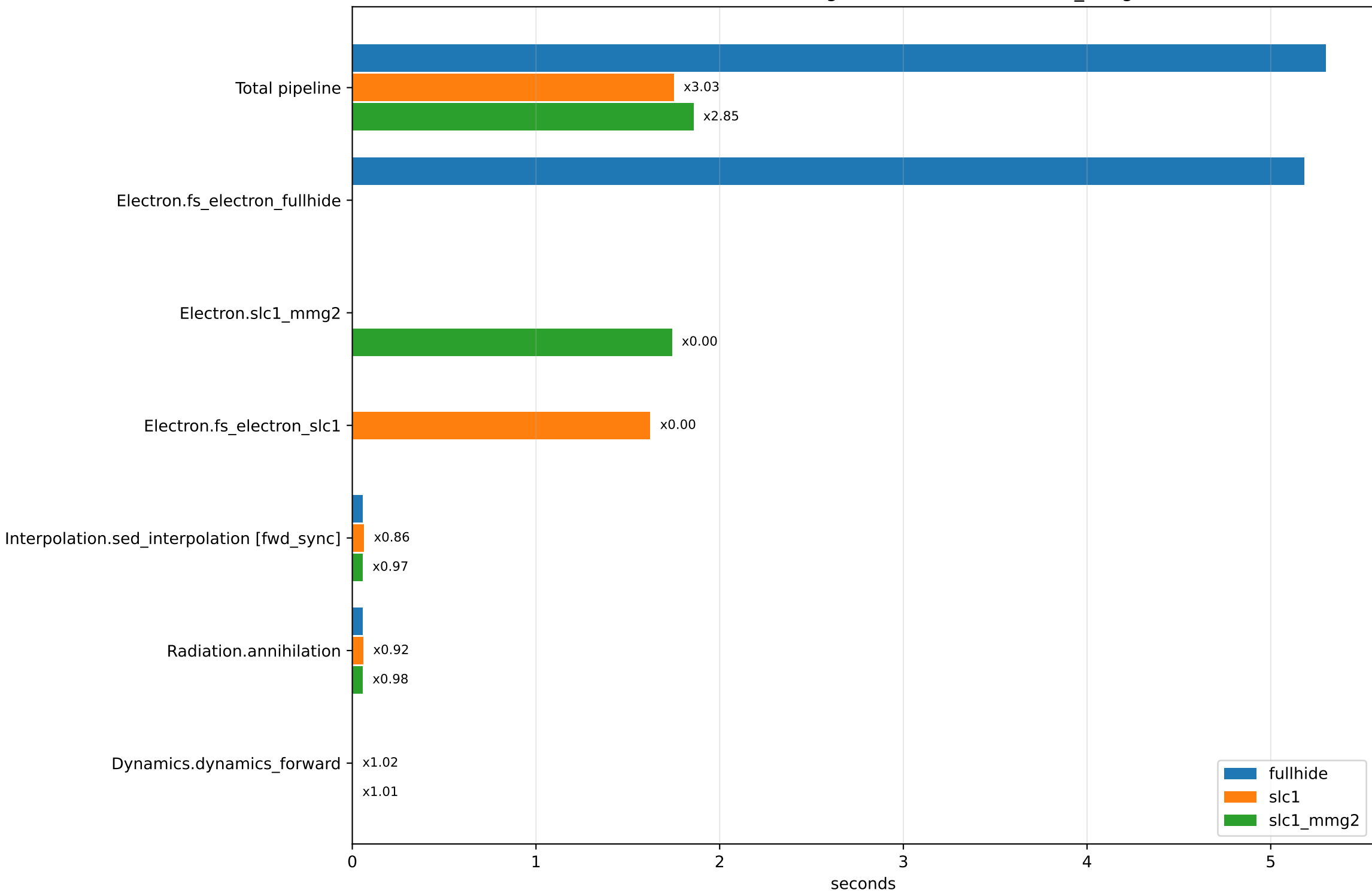
ASGARD subroutine timings: fullhide vs slc1 vs slc1_mmg2
