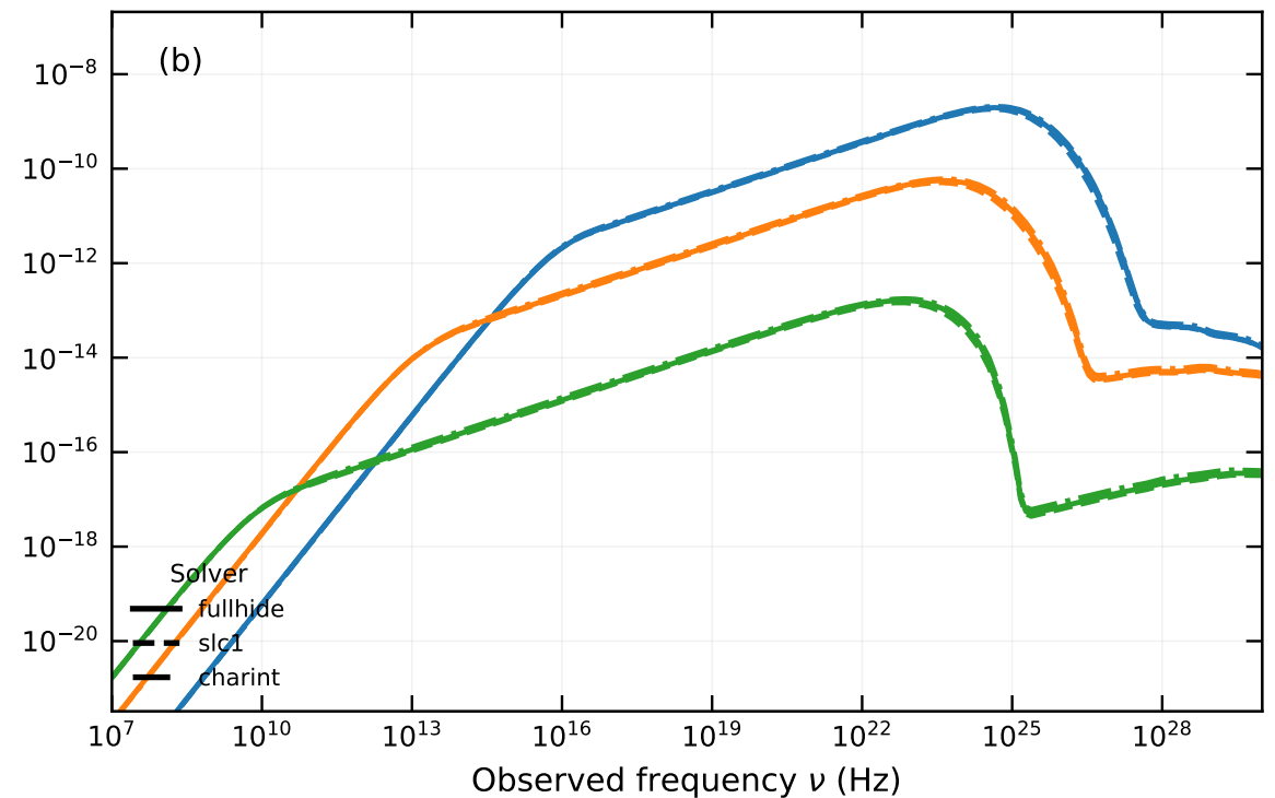
WIND Forward Shock
