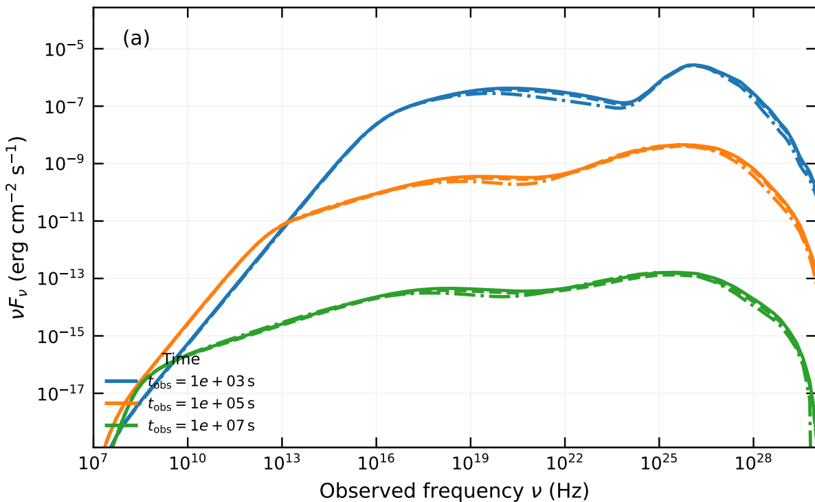
ISM Forward Shock
