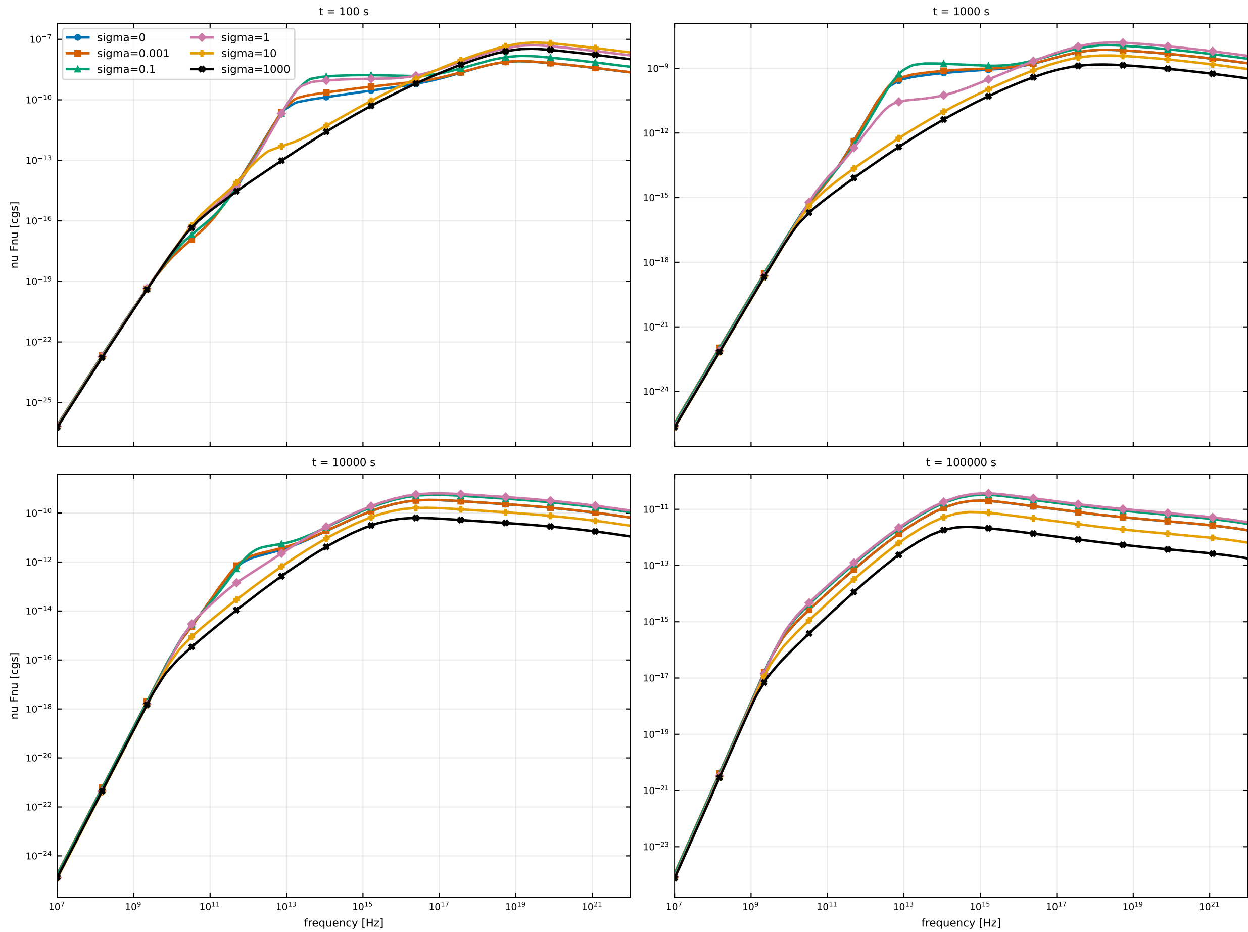
ASGARD magnetized RS sigma scan (ism, nakar_y_thomson): total SED
