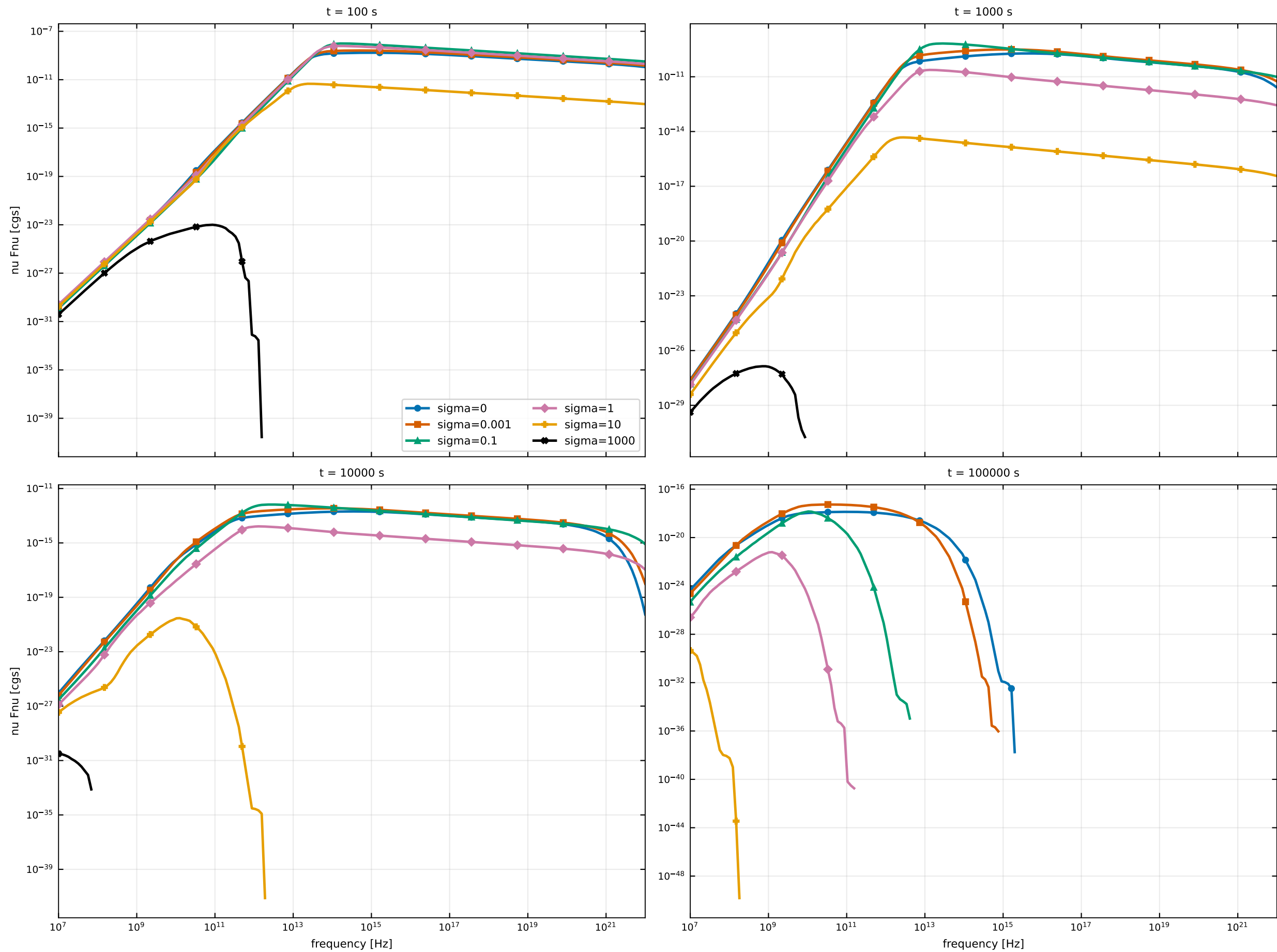
ASGARD magnetized RS sigma scan (wind, nakar_y_thomson): RS synch SED
