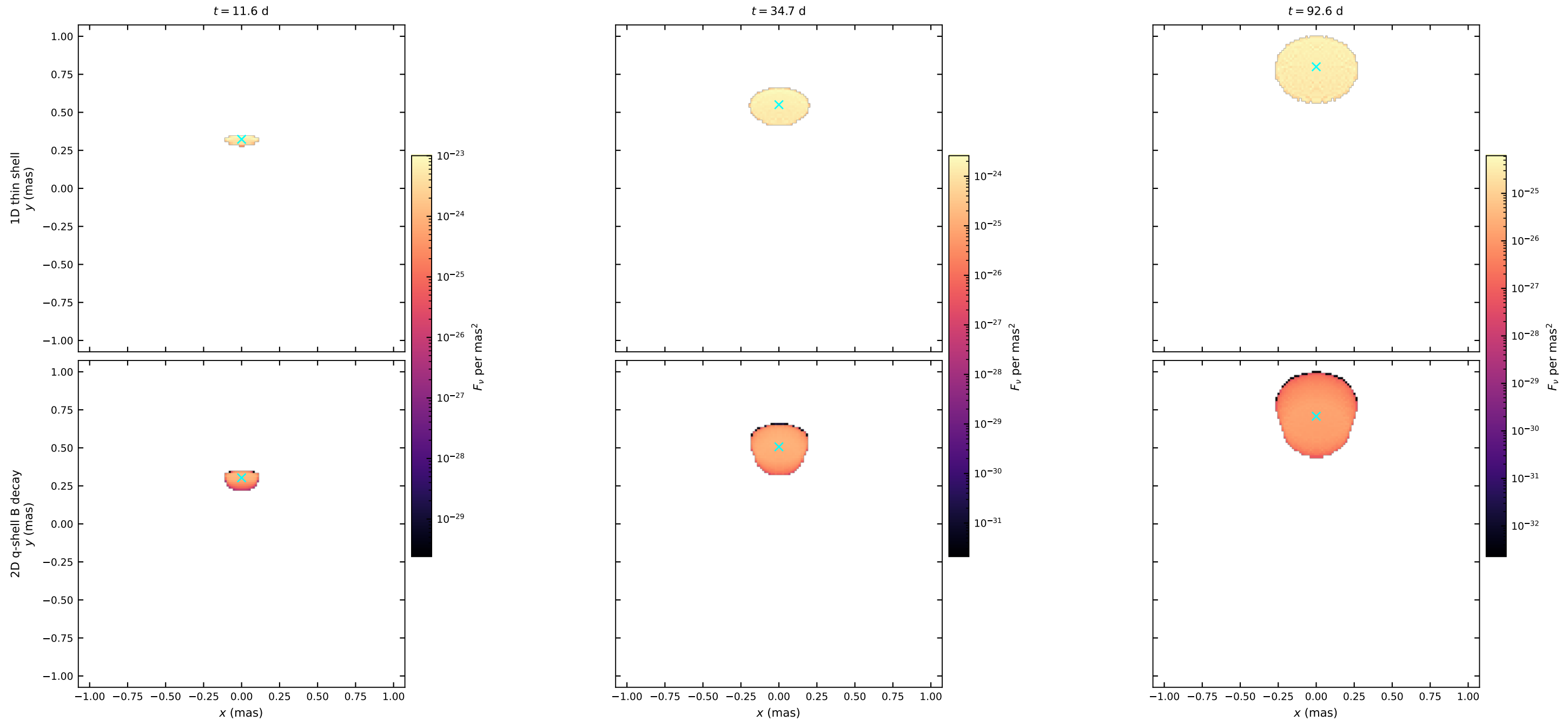
Sky maps at \nu = 1\text{e} + 10\text{ Hz} , \theta_\nu/\theta_j = 3
