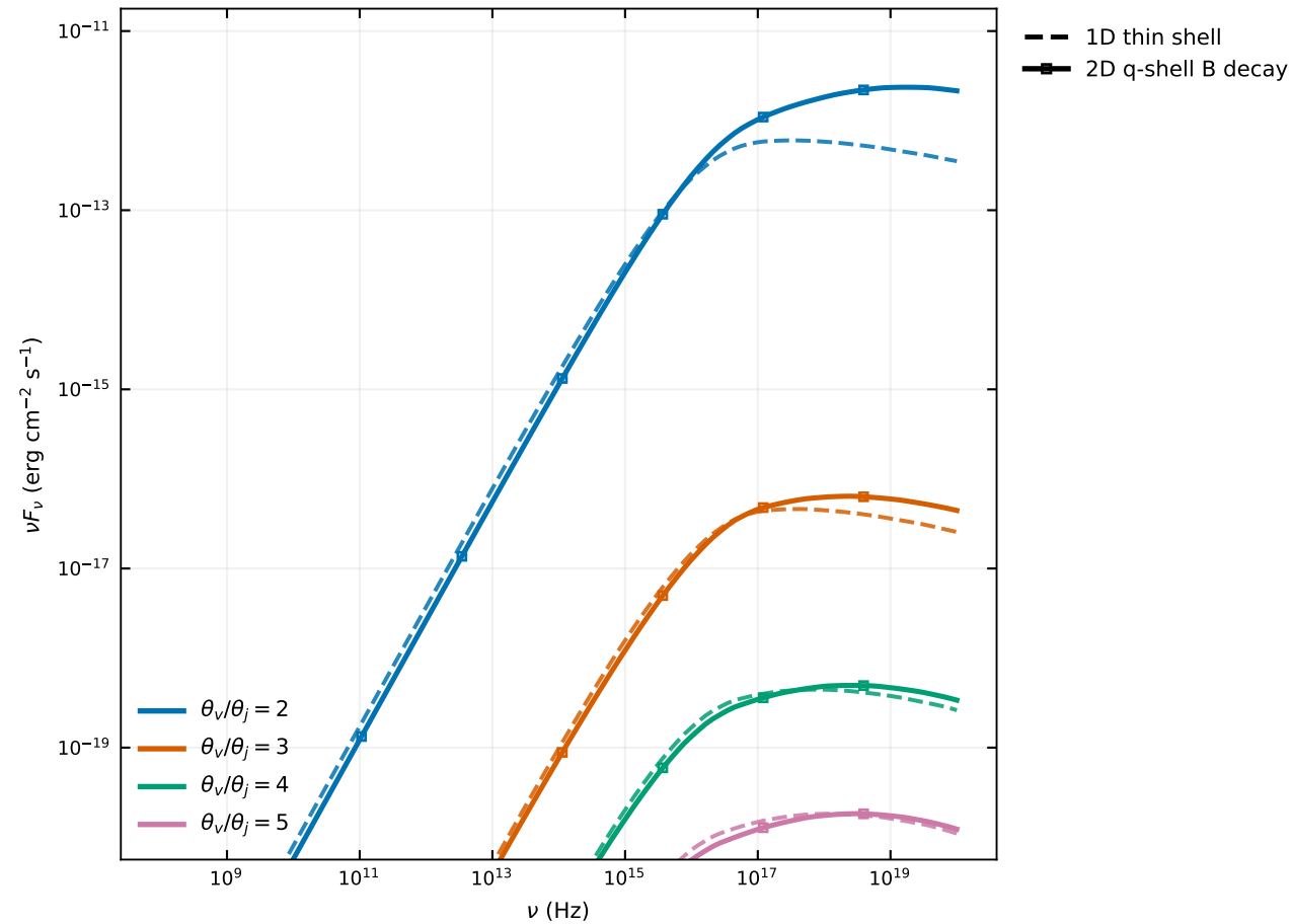
Spectrum at t_{\text{obs}} = 10^4 s
