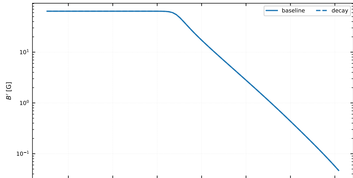
\alpha_t = -0.5 , t'_0 = 1.0e + 02 s, \epsilon_{B, \text{floor}}/\epsilon_{B, +} = 1.0e - 03
