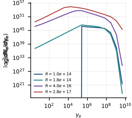
b Injection, cooling, aging
