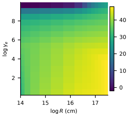
a Electron transport history
