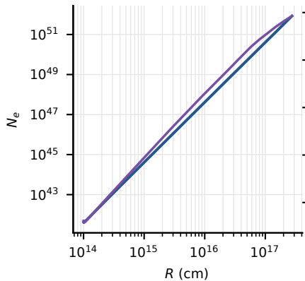
c Number and energy budgets
