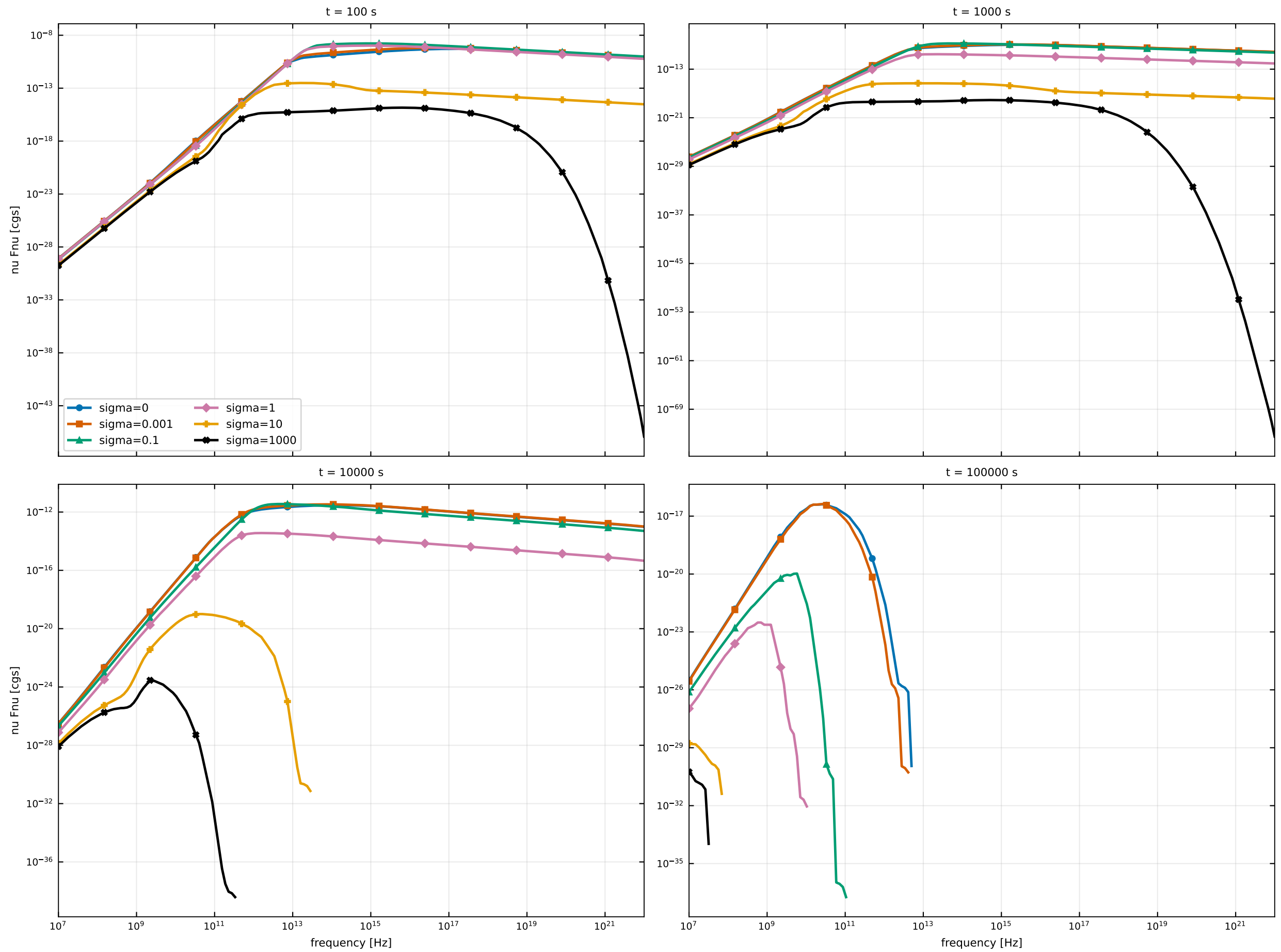
ASGARD magnetized RS sigma scan (ism, nakar_y_thomson): RS synch SED
