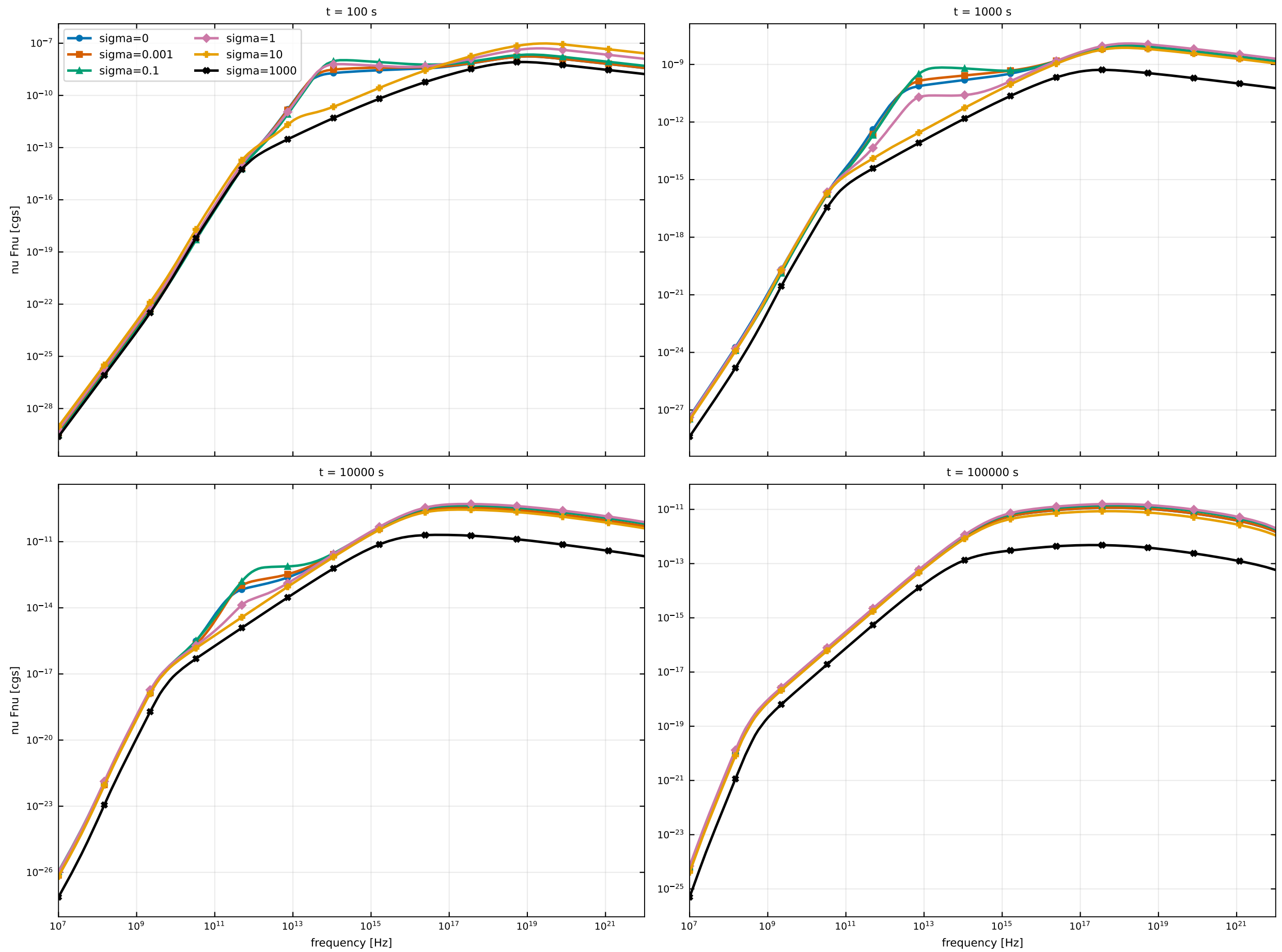
ASGARD magnetized RS sigma scan (wind, nakar_y_thomson): total SED
