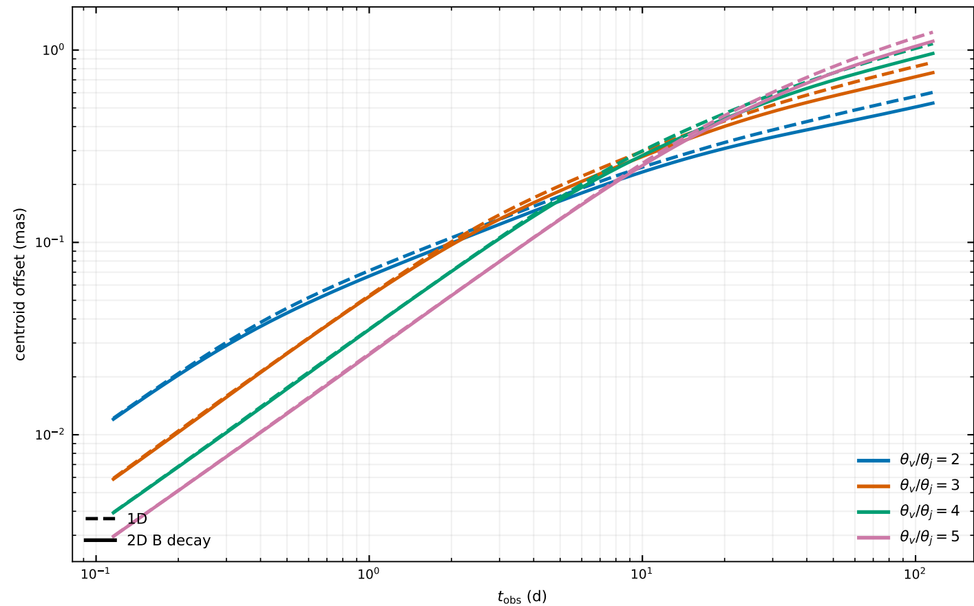
Flux-centroid offset at \nu = 1\text{e} + 10\text{ Hz}
