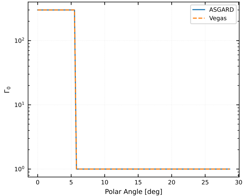
Jet Initial Lorentz Factor
