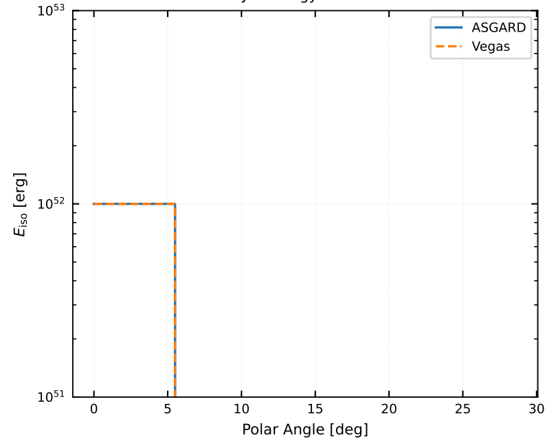
Jet Energy Profile
