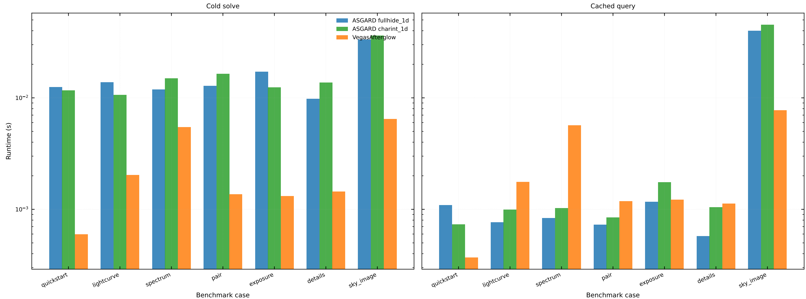
Speed profile: explicit first solve and warmed-cache query
