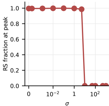
b RS contribution
