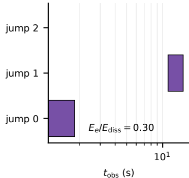
c Secondary RS windows
