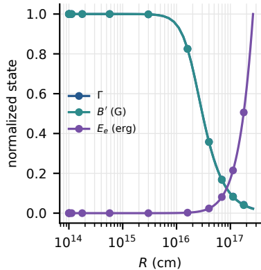
c Full state chain
