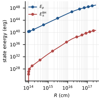
a Hadronic and pair state
