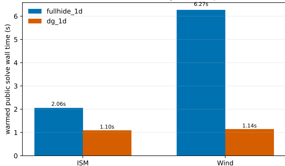
BE+10 DG multi-band light-curve speed
