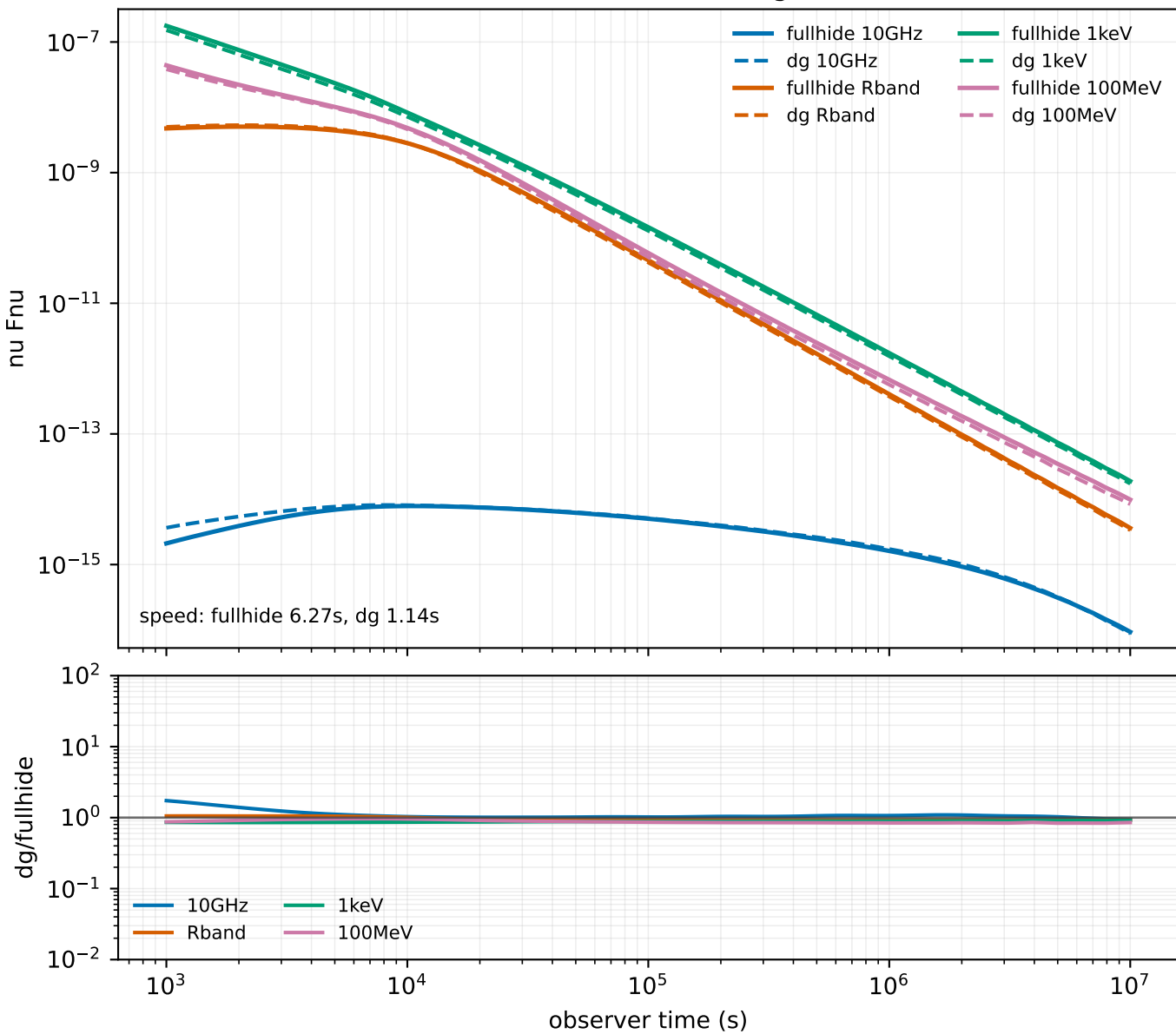
BE+10 DG vs fullhide multi-band light curves: Wind
