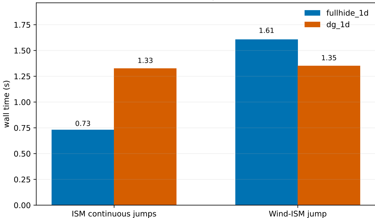
0.1-1e7 s multi-band light-curve solve time
