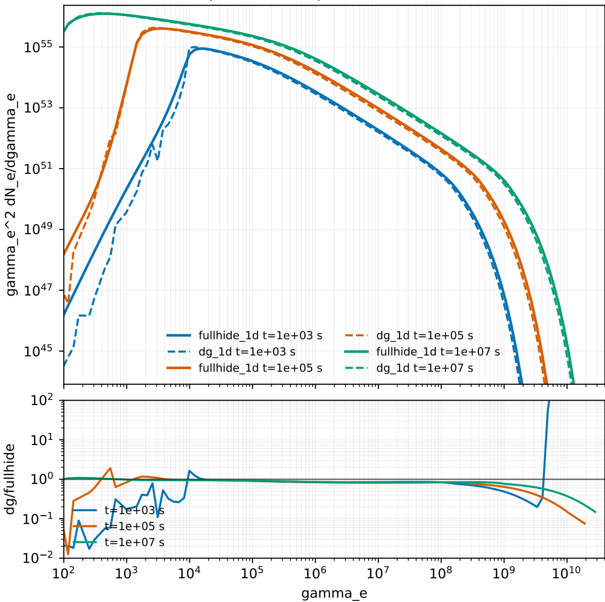
Electron spectrum comparison: ISM Forward Shock
