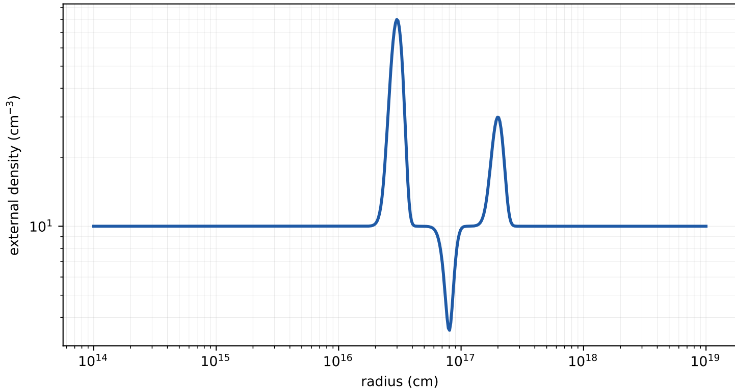
ISM continuous density jumps, relative width 0.1
