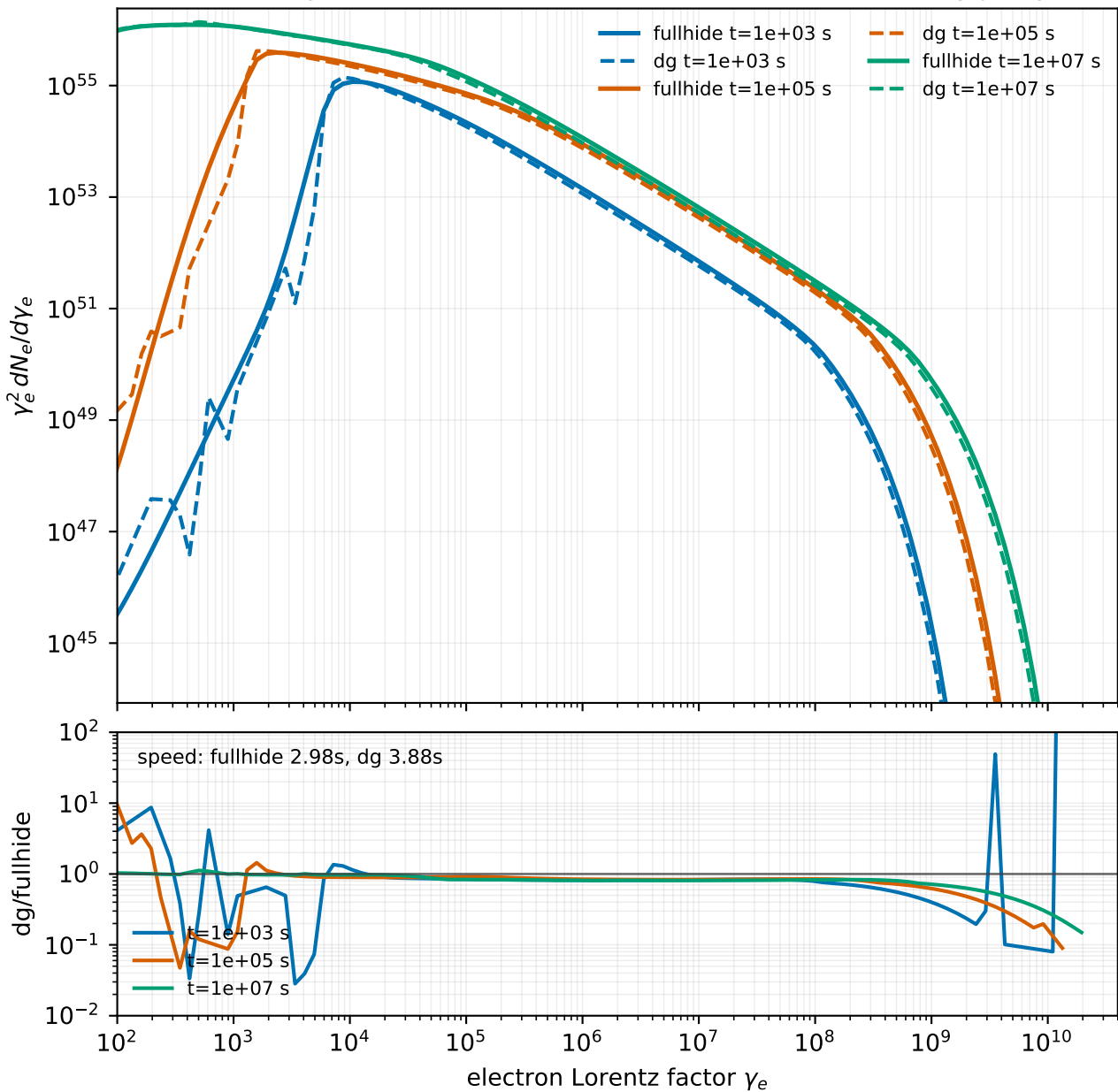
Electron spectrum: Tabulated medium with three density jumps
