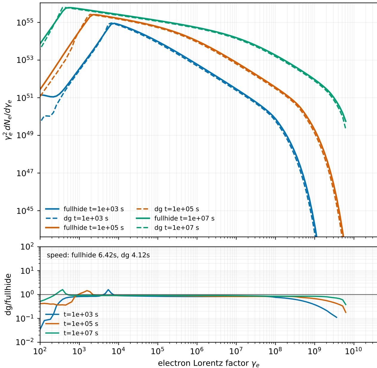
Electron spectrum: Wind medium
