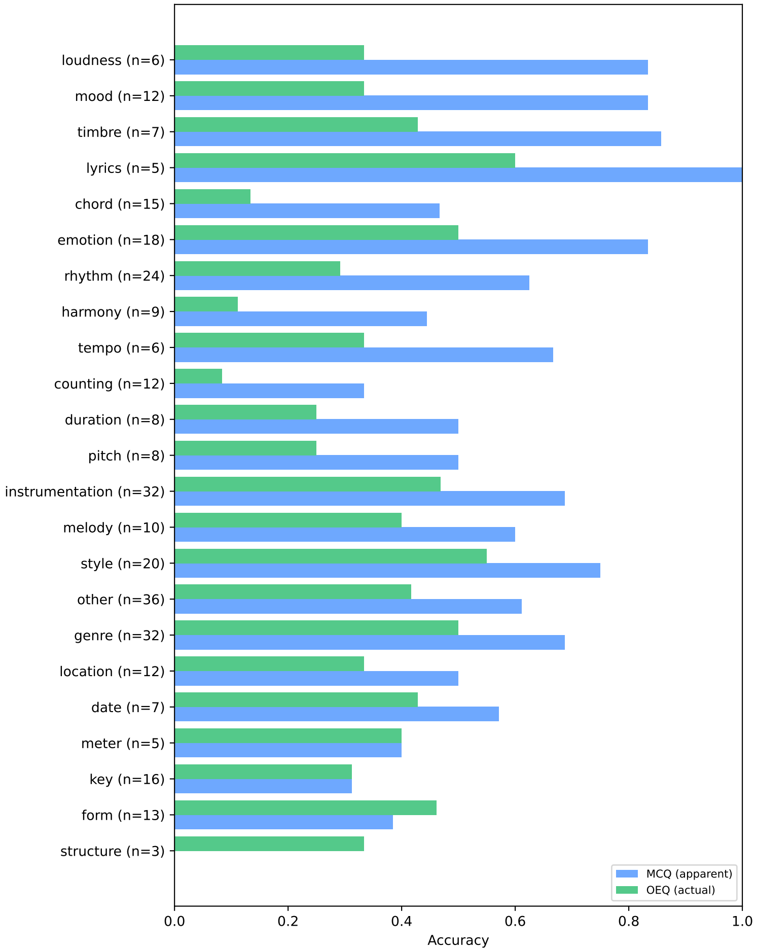
Apparent (MCQ) vs actual (OEQ) accuracy by skill
