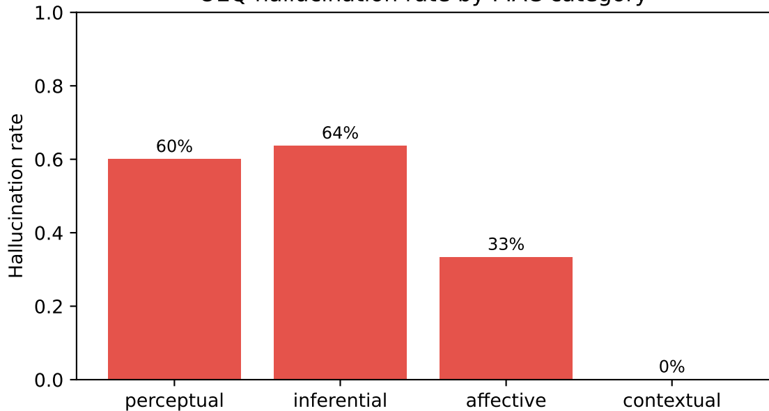
OEQ hallucination rate by PIAC category
