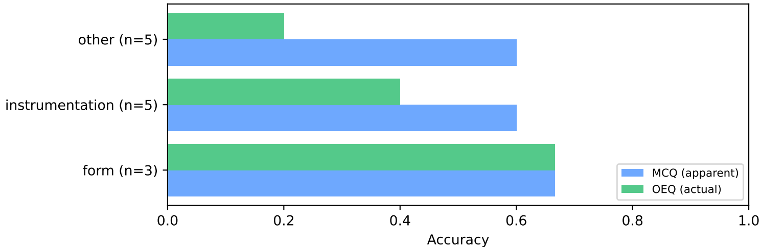
Apparent (MCQ) vs actual (OEQ) accuracy by skill
