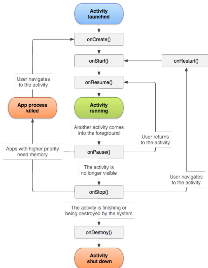
Figure 2.1: Activity lifecycle Android[4]
