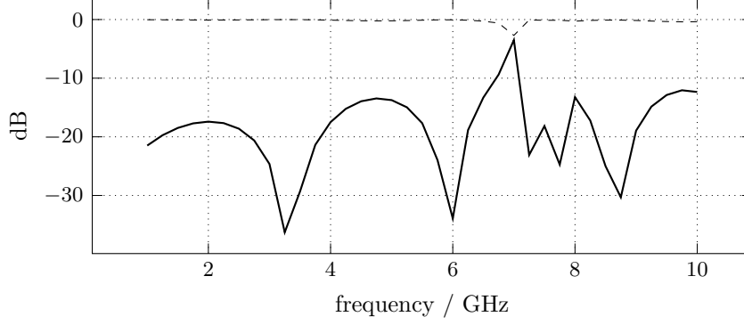
Figure 9: Reflection, solid, and transmission, dashed, of the line. Reflection stays below -12 dB from 1 to 10 GHz apart from a peak at 7 GHz, where |S_{11}| reaches -3.5 dB and |S_{21}| falls to -2.7 dB. Narrowing the enclosure from 20 to 16 mm removes that peak and puts a similar one at 9 GHz, so it belongs to the box and not to the line.
