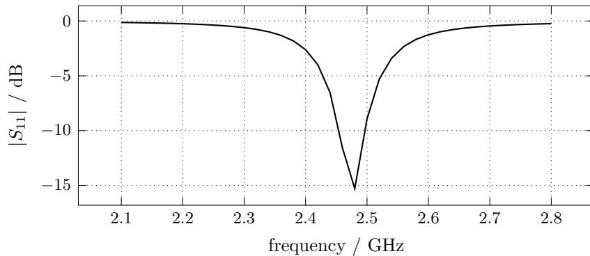
Figure 6: Reflection of the reference antenna. The resonance appears as a dip at 2.48 GHz on this mesh, against a design value of 2.45 GHz. Refining the mesh moves it to 2.50 GHz, so the discretization error is still the largest term.
