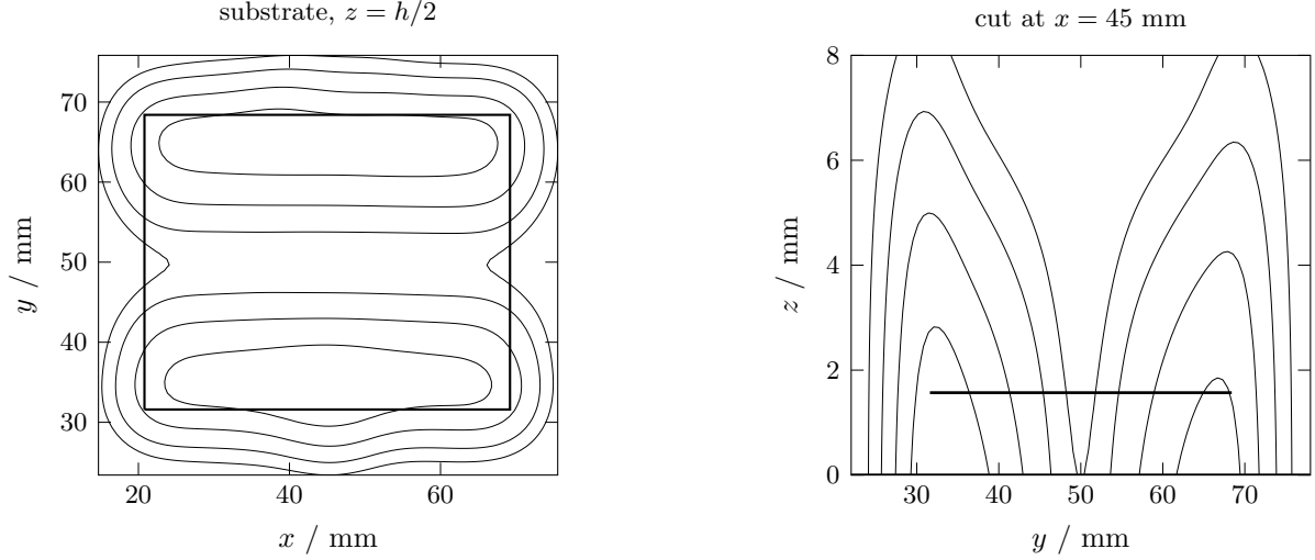
Figure 7: Contours of the electric field magnitude at the resonance, at -11 , -7 , -4 and -2 dB below the peak of each cut. Left, a horizontal cut through the middle of the substrate with the patch outline drawn: the field is confined under the patch and forms the half wave along y that sets the resonant length, with maxima at the two radiating edges and a null across the middle. Right, a vertical cut along the resonant direction through the middle of the patch, with the ground plane and the patch as the heavy lines: the same half wave appears in the substrate, and the field that escapes past the two patch edges is the fringing that radiates.
