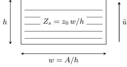
Figure 5: A lumped port. The patch of boundary triangles carries a sheet impedance and an impressed surface current. Its height is the extent of the patch along the given direction \hat{u} and its width follows from the total area, so the deck states only \hat{u} and the reference impedance z_0 .
