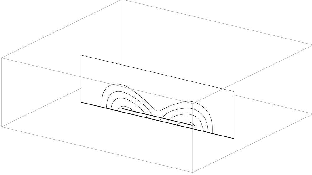
Figure 8: A vertical cut of the same field on the plane the mesh is cut at. The view, the scale and the outlined box are those of figure 6, so every figure of this model is the same scene seen from the same place. The plane is opaque and the box outline is cut against it. Contours at -17.5 , -12.5 , -7.5 and -2.5 dB below the peak of the cut. The heavy lines are the ground plane and the patch. The half wave appears again in the substrate, and the two lobes reaching into the air past the patch edges are the fringing that radiates.
