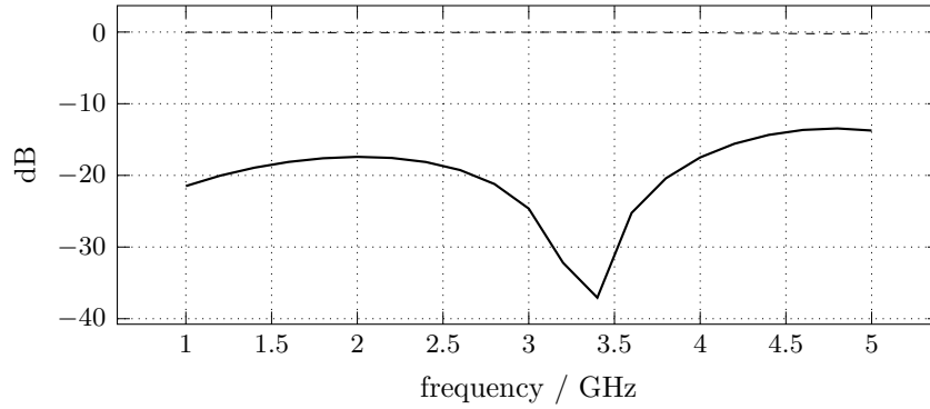
Figure 13: Reflection, solid, and transmission, dashed, of the line. Reflection stays between -13 and -37 dB over the band and transmission above -0.3 dB.
