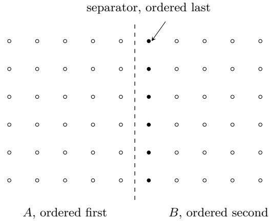
Figure 3: One level of the geometric nested dissection. The unknowns are split at the median of the longest bounding box axis. Those on the second side with a neighbour on the first form the separator and are numbered after both halves, so no fill can connect A to B . Both halves are then split recursively down to blocks of 32.
