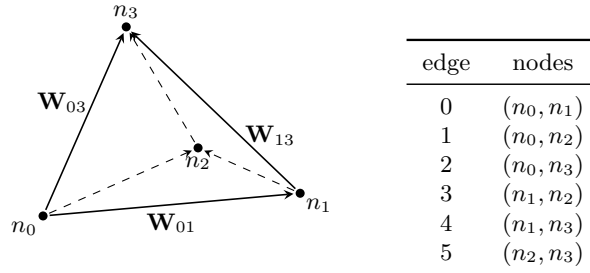
Figure 2: The six edge unknowns of a tetrahedron and the local edge table the code uses. The unknown on an edge is the line integral of \mathbf{E} along it. Node indices are sorted on input, so every arrow runs from the lower to the higher global index and two tetrahedra sharing an edge assign it the same direction without a sign convention. Edges meeting the rear node n_2 are dashed.
