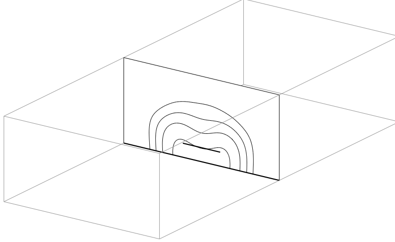
Figure 12: A vertical cut of the same field on the plane the mesh is cut at. The view, the scale and the outlined box are those of figure 10, so every figure of this model is the same scene seen from the same place. The plane is opaque and the box outline is cut against it. Contours at -17.5 , -12.5 , -7.5 and -2.5 dB below the peak of the cut. The heavy lines are the ground plane and the strip. The field fills the substrate under the strip, fringes past its two edges and is 25 dB down at the side walls and the lid.
