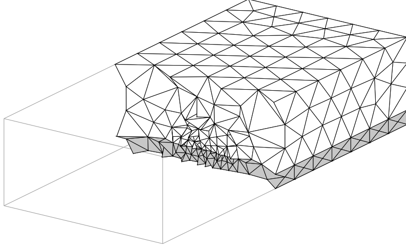
Figure 10: The mesh, cut at x = 22 mm halfway along the line and drawn back to front with opaque faces, inside the outline of the full domain. What the cut took away stays visible as the empty half of the box. The dark layer at the bottom is the substrate; this model has no absorbing layer.
