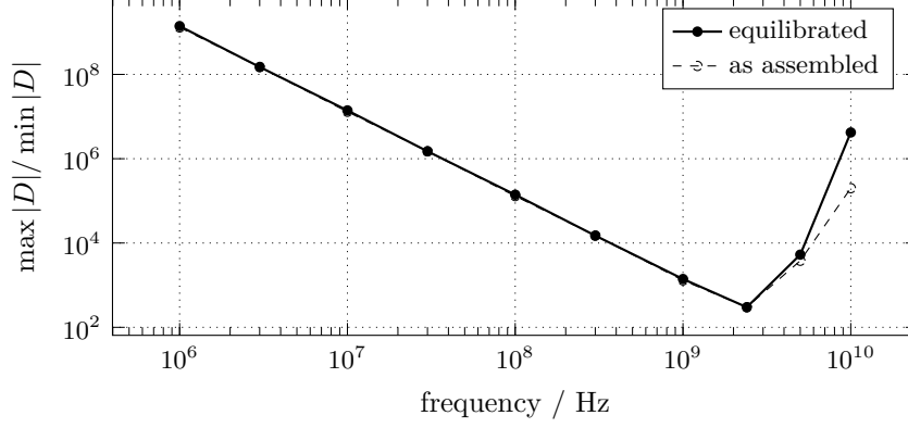
Figure 4: Pivot spread of the reference antenna against frequency. The 1/f^2 branch on the left is the low frequency breakdown of the curl-curl operator, which loses the mass term that regularizes its nullspace. The rise on the right sets in once the mesh becomes coarse against the wavelength. Equilibration gains a factor of about three over the low frequency branch and about four in the operating band.
