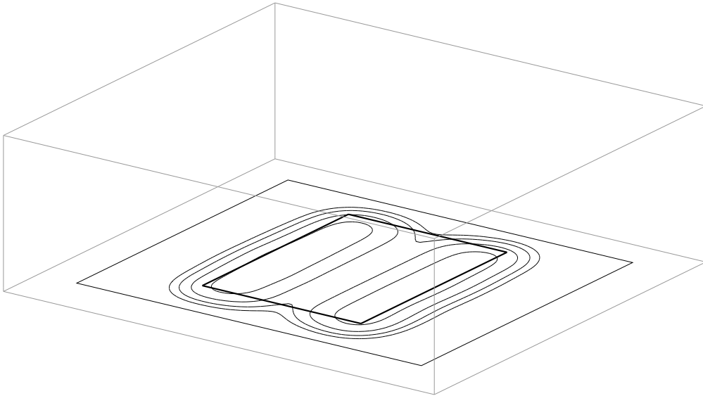
Figure 7: A horizontal cut of the electric field magnitude through the middle of the substrate, at the resonance. The view, the scale and the outlined box are those of figure 6, so every figure of this model is the same scene seen from the same place. The plane is opaque and the box outline is cut against it. Contours at -17.5 , -12.5 , -7.5 and -2.5 dB below the peak of the cut. The heavy rectangle is the patch. The field is confined under it and forms the half wave along y that sets the resonant length, with maxima at the two radiating edges and a null across the middle.
