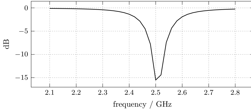
Figure 9: Reflection of the antenna. The resonance appears as a dip at 2.50 GHz, against a design value of 2.45 GHz. A mesh coarsened by a factor of one and a half puts it at 2.48 GHz, so the discretization error is still the largest term.
