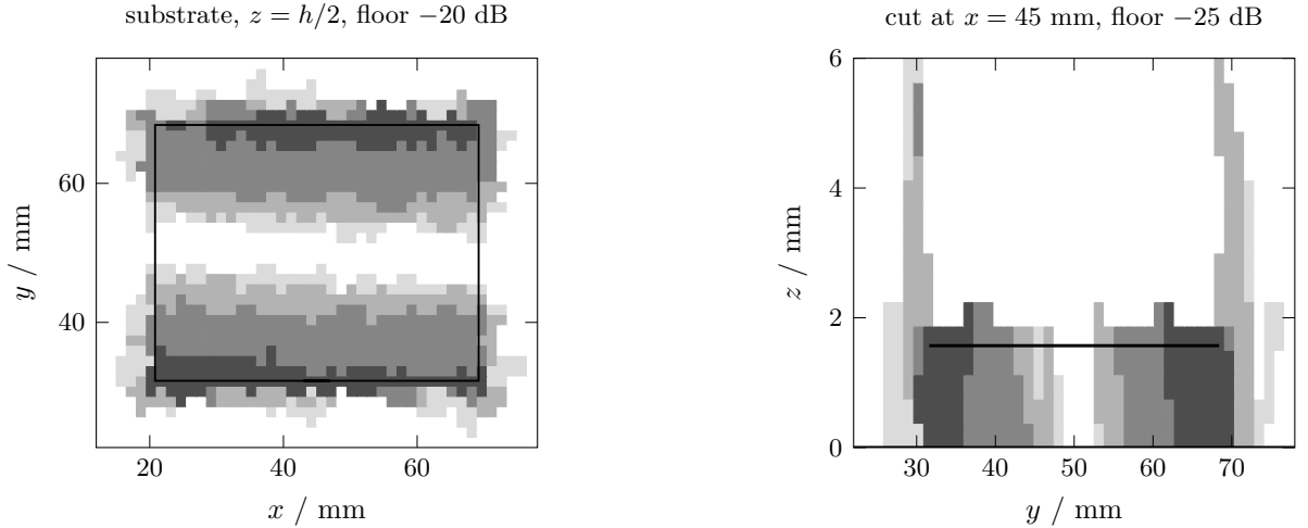
Figure 6: Magnitude of the electric field at 2.4 GHz with the port driven, on six grey levels of a decibel scale relative to the peak of each cut. Left, a horizontal cut through the middle of the substrate with the patch outline and the feed drawn: the field is confined under the patch and forms the half wave variation along y that sets the resonant length, with maxima at the two radiating edges and a null across the middle. Right, a vertical cut along the resonant direction through the middle of the patch, with the ground plane and the patch as the heavy lines: the same half wave appears in the substrate, and the field that escapes past the two patch edges is the fringing that radiates.
