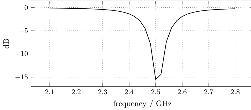
Figure 8: Reflection of the antenna. The resonance appears as a dip at 2.50 GHz, against a design value of 2.45 GHz. A mesh coarsened by a factor of one and a half puts it at 2.48 GHz, so the discretization error is still the largest term.
