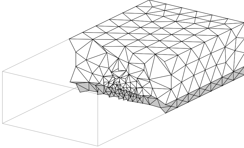
Figure 9: The mesh, cut at x = 22 mm halfway along the line and drawn back to front with opaque faces, inside the outline of the full domain. What the cut took away stays visible as the empty half of the box. The dark layer at the bottom is the substrate; this model has no absorbing layer.
