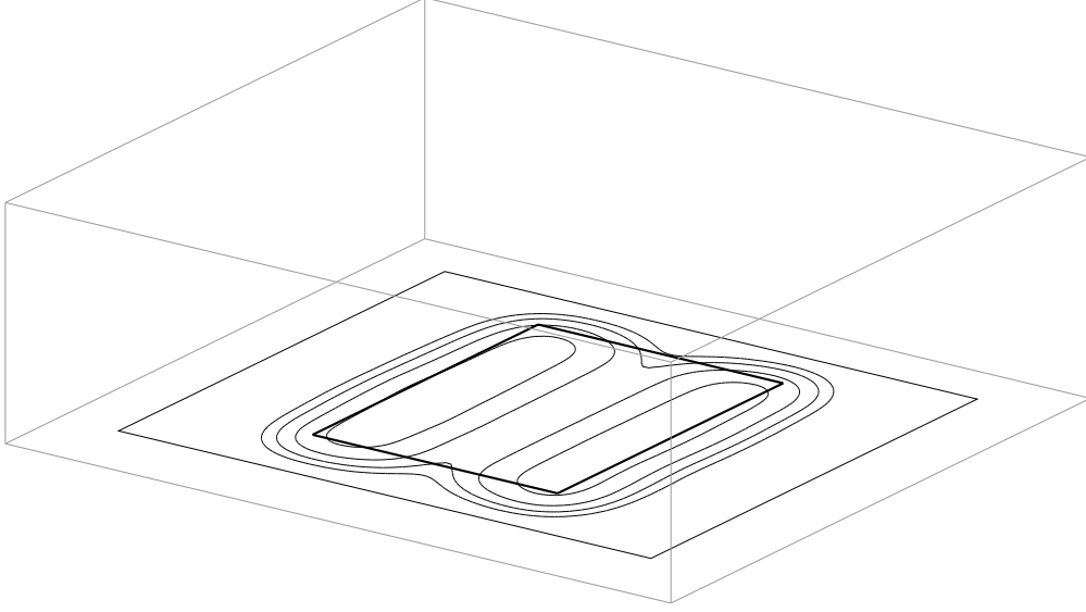
Figure 6: A horizontal cut of the electric field magnitude through the middle of the substrate, at the resonance. The view, the scale and the outlined box are those of figure 5, so every figure of this model is the same scene seen from the same place. The plane is opaque and the box outline is cut against it. Contours at -17.5 , -12.5 , -7.5 and -2.5 dB below the peak of the cut. The heavy rectangle is the patch. The field is confined under it and forms the half wave along y that sets the resonant length, with maxima at the two radiating edges and a null across the middle.
