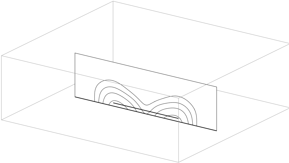
Figure 7: A vertical cut of the same field on the plane the mesh is cut at. The view, the scale and the outlined box are those of figure 5, so every figure of this model is the same scene seen from the same place. The plane is opaque and the box outline is cut against it. Contours at -17.5 , -12.5 , -7.5 and -2.5 dB below the peak of the cut. The heavy lines are the ground plane and the patch. The half wave appears again in the substrate, and the two lobes reaching into the air past the patch edges are the fringing that radiates.
