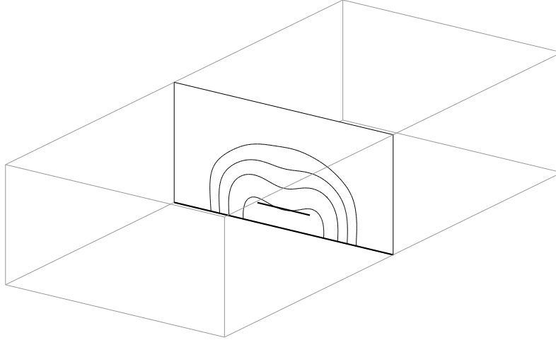
Figure 11: A vertical cut of the same field on the plane the mesh is cut at. The view, the scale and the outlined box are those of figure 9, so every figure of this model is the same scene seen from the same place. The plane is opaque and the box outline is cut against it. Contours at -17.5 , -12.5 , -7.5 and -2.5 dB below the peak of the cut. The heavy lines are the ground plane and the strip. The field fills the substrate under the strip, fringes past its two edges and is 25 dB down at the side walls and the lid.
