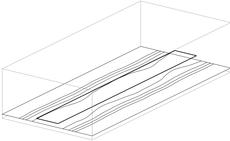
Figure 10: A horizontal cut of the electric field magnitude through the middle of the substrate, at 5 GHz. The view, the scale and the outlined box are those of figure 9, so every figure of this model is the same scene seen from the same place. The plane is opaque and the box outline is cut against it. Contours at -17.5 , -12.5 , -7.5 and -2.5 dB below the peak of the cut. The heavy rectangle is the strip. The field is confined under it along the whole length of the line, which is what a uniform line carrying one mode looks like.
