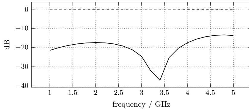
Figure 12: Reflection, solid, and transmission, dashed, of the line. Reflection stays between -13 and -37 dB over the band and transmission above -0.3 dB.
