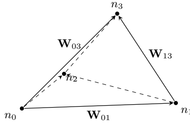
Figure 1: The six edge unknowns of a tetrahedron. The unknown on an edge is the line integral of \mathbf{E} along it. Node indices are sorted on input, so every arrow runs from the lower to the higher global index and two tetrahedra sharing an edge assign it the same direction without a sign convention. Dashed edges are behind the front face.
