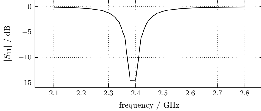
Figure 5: Reflection of the reference antenna. The resonance appears as a dip near 2.4 GHz on this mesh. It is not converged: refining the mesh moves it to 2.48 GHz, and part of the remaining drift is the first order absorbing boundary, which sits about a third of a wavelength above the patch.
