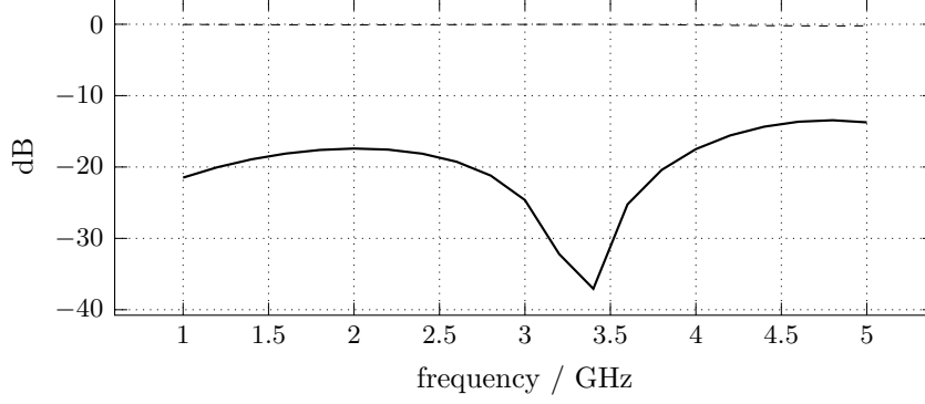
Figure 9: Reflection, solid, and transmission, dashed, of the line. Reflection stays between -13 and -37 dB over the band and transmission above -0.3 dB.
