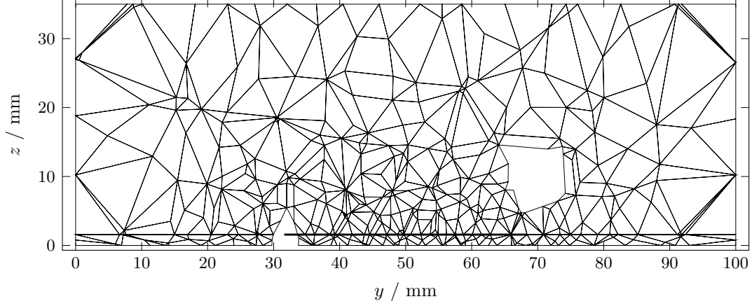
Figure 5: The tetrahedral mesh cut by the plane x = 45 mm, the same plane as the right hand field map. The substrate is the flat layer of elements below z = 1.57 mm and the patch is the heavy line on top of it. The element size is set by a distance field on the patch and the feed, growing from 3 mm at the metal to 11 mm at the far corners of the air box, so the aspect ratio stays bounded through the transition out of the substrate. A uniform maximum size instead produces slivers spanning the air region and moves the resonance by two percent.
