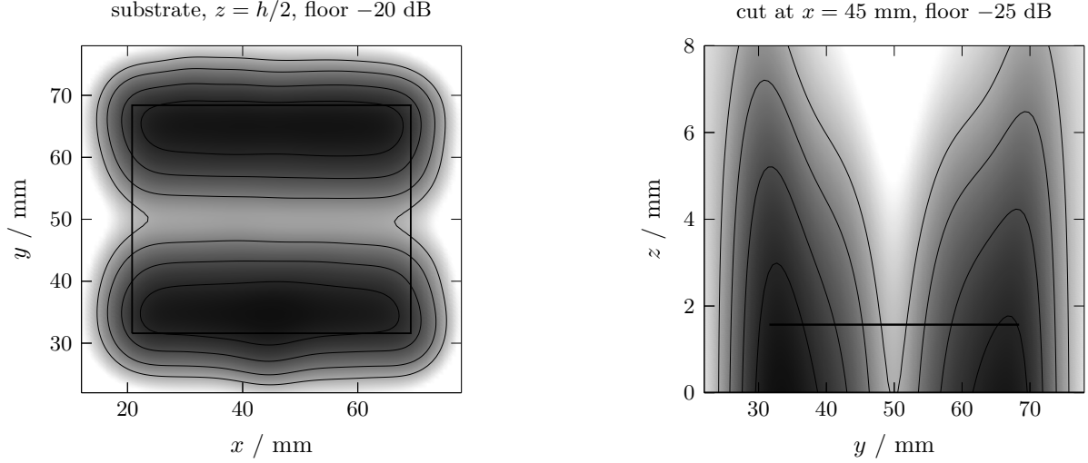
Figure 7: Magnitude of the electric field at the resonance, 2.45 GHz, with the port driven, on a decibel scale relative to the peak of each cut and contours at -11 , -7 , -4 and -2 dB of the range. Left, a horizontal cut through the middle of the substrate with the patch outline drawn: the field is confined under the patch and forms the half wave along y that sets the resonant length, with maxima at the two radiating edges and a null across the middle. Right, a vertical cut along the resonant direction through the middle of the patch, with the ground plane and the patch as the heavy lines: the same half wave appears in the substrate, and the field that escapes past the two patch edges is the fringing that radiates.
