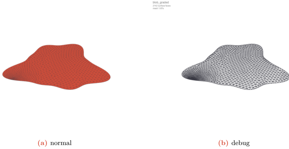
Figure 16: blob_graded (Sizing): normal view (left, region-coloured, volumes clipped) and debug view (right, defect markers and per-stage timing). 2142 triangles.
