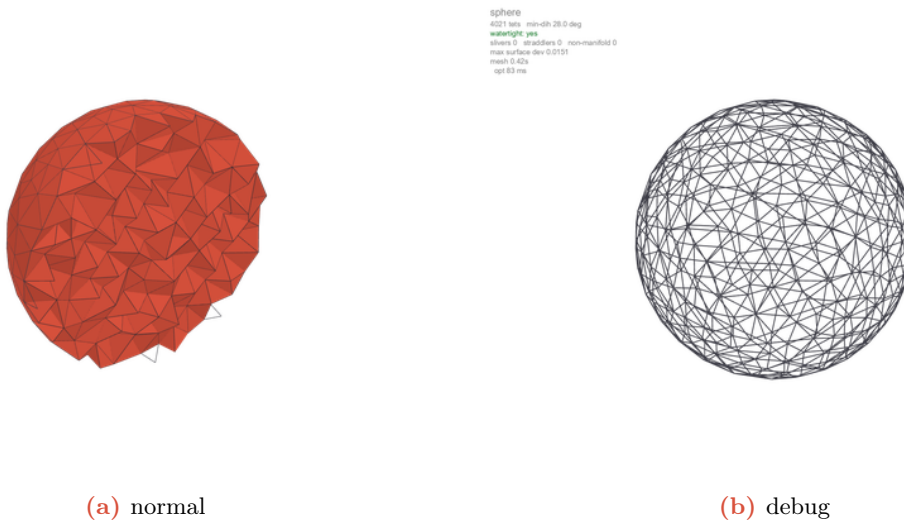
Figure 7: sphere (Analytic primitives): normal view (left, region-coloured, volumes clipped) and debug view (right, defect markers and per-stage timing). 4021 tets, min dihedral 28.0^\circ , watertight.
