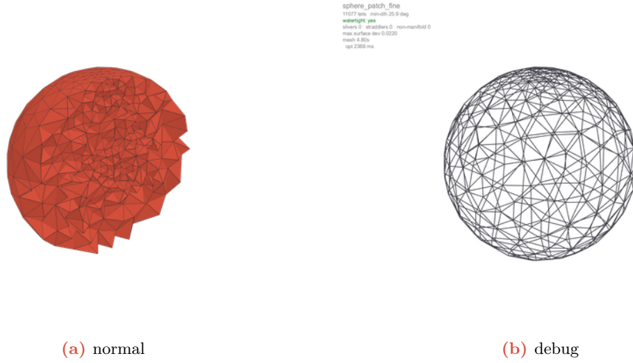
Figure 20: sphere_patch_fine (Graded): normal view (left, region-coloured, volumes clipped) and debug view (right, defect markers and per-stage timing). 11077 tets, min dihedral 25.9^\circ , watertight.
