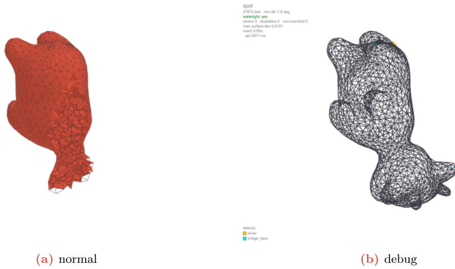
Figure 11: spot (Imported reference models (discrete carriers)): normal view (left, region-coloured, volumes clipped) and debug view (right, defect markers and per-stage timing). 27873 tets, min dihedral 7.8^\circ , watertight, 3 slivers, 2 bridge faces.
