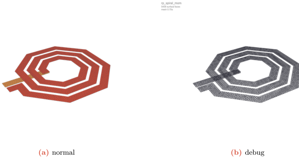
Figure 21: rp_spiral_mom (Passives): normal view (left, region-coloured, volumes clipped) and debug view (right, defect markers and per-stage timing). 5458 triangles.
