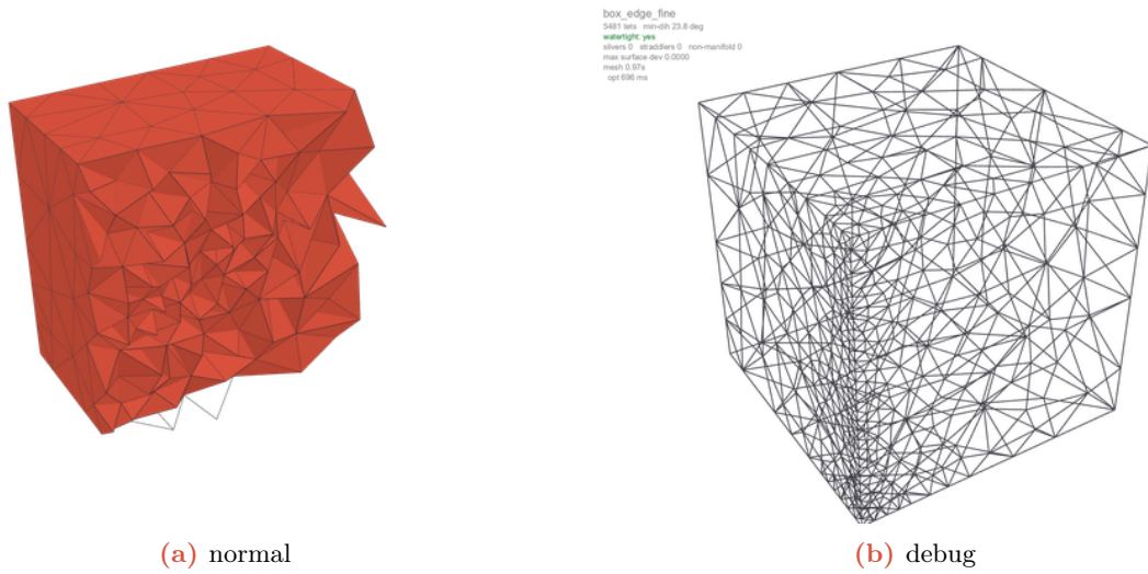
Figure 19: box_edge_fine (Graded): normal view (left, region-coloured, volumes clipped) and debug view (right, defect markers and per-stage timing). 5481 tets, min dihedral 23.8^\circ , watertight.
