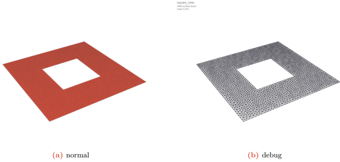
Figure 4: square_hole (2D plates (planar surface stage)): normal view (left, region-coloured, volumes clipped) and debug view (right, defect markers and per-stage timing). 4498 triangles.
