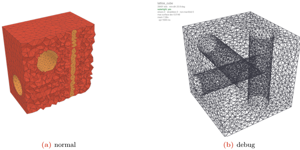
Figure 13: lattice_cube (Showcase models): normal view (left, region-coloured, volumes clipped) and debug view (right, defect markers and per-stage timing). 39491 tets, min dihedral 20.8^\circ , watertight.
