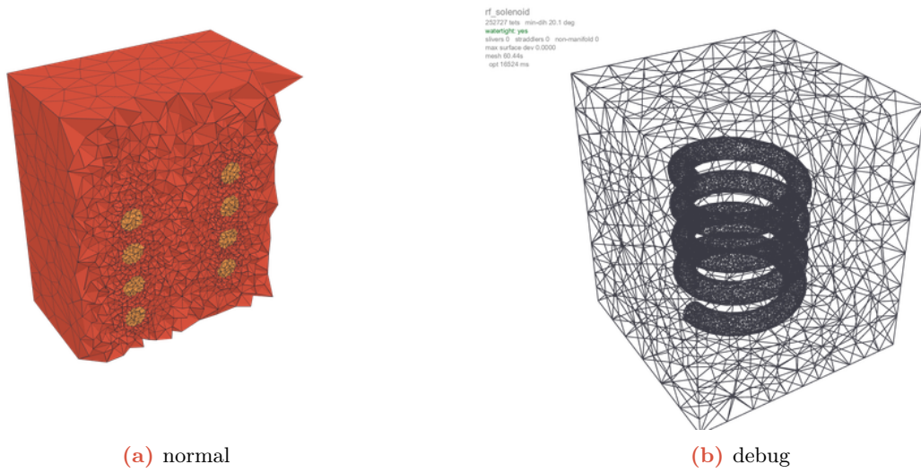
Figure 15: rf_solenoid (RF/EM structures): normal view (left, region-coloured, volumes clipped) and debug view (right, defect markers and per-stage timing). 252727 tets, min dihedral 20.1^\circ , watertight.
