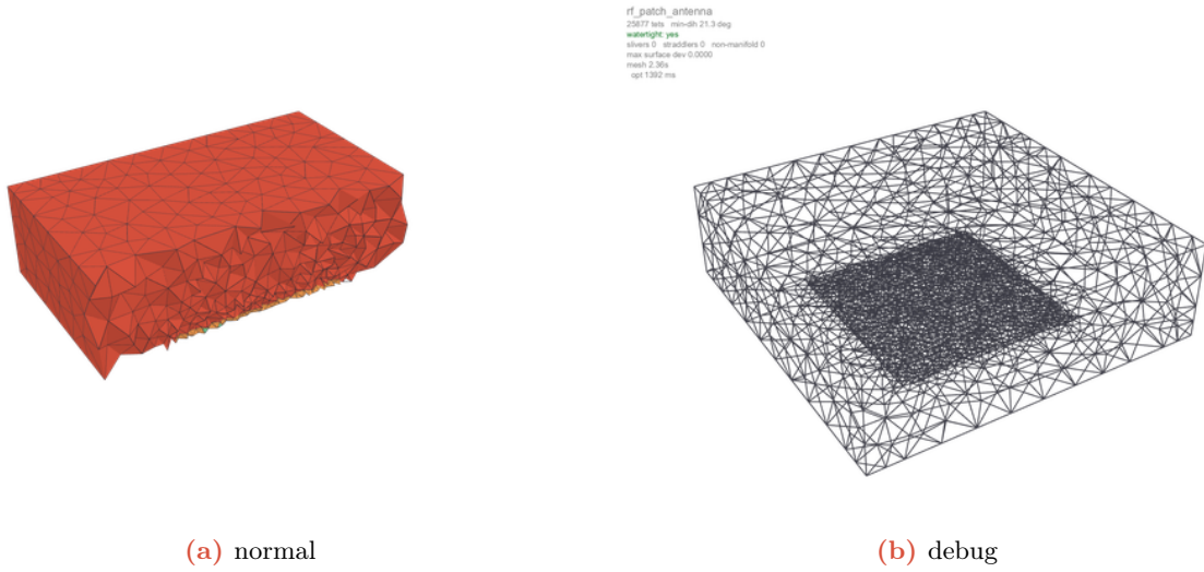
Figure 14: rf_patch_antenna (RF/EM structures): normal view (left, region-coloured, volumes clipped) and debug view (right, defect markers and per-stage timing). 25877 tets, min dihedral 21.3^\circ , watertight.
