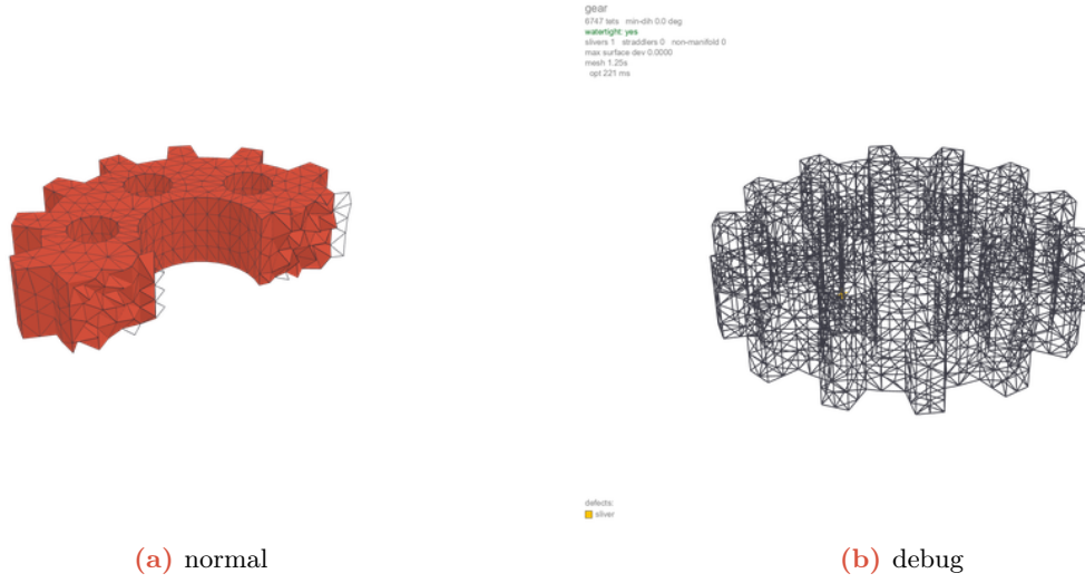
Figure 12: gear (Showcase models): normal view (left, region-coloured, volumes clipped) and debug view (right, defect markers and per-stage timing). 6747 tets, min dihedral 0.0^\circ , watertight, 1 slivers.
