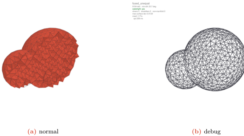
Figure 9: fused_unequal (CSG booleans and multi-region assemblies): normal view (left, region-coloured, volumes clipped) and debug view (right, defect markers and per-stage timing). 9194 tets, min dihedral 20.7^\circ , watertight.
