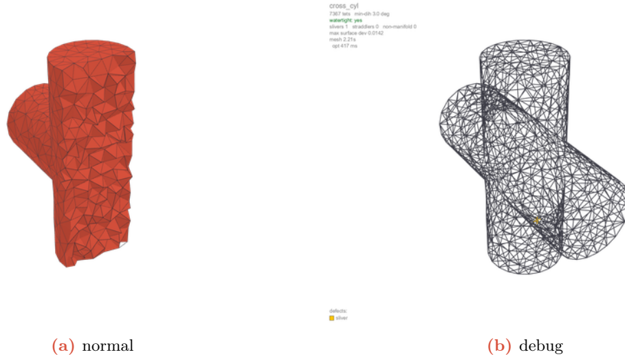
Figure 8: cross_cyl (CSG booleans and multi-region assemblies): normal view (left, region-coloured, volumes clipped) and debug view (right, defect markers and per-stage timing). 7367 tets, min dihedral 3.0^\circ , watertight, 1 slivers.
