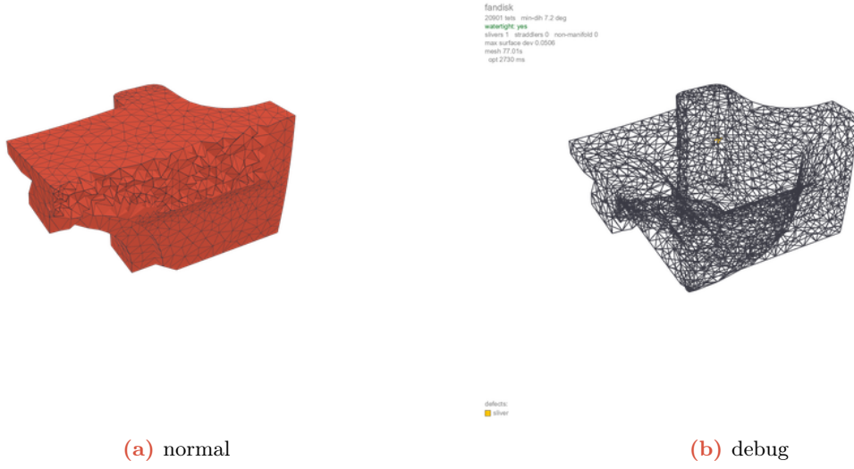
Figure 10: fandisk (Imported reference models (discrete carriers)): normal view (left, region-coloured, volumes clipped) and debug view (right, defect markers and per-stage timing). 20901 tets, min dihedral 7.2^\circ , watertight, 1 slivers.
