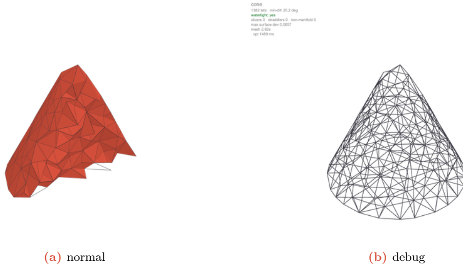
Figure 6: cone (Analytic primitives): normal view (left, region-coloured, volumes clipped) and debug view (right, defect markers and per-stage timing). 1382 tets, min dihedral 20.2^\circ , watertight.
