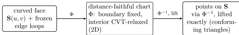
Figure 3: Surface meshing through a chart: relax in a (near-)isometric 2D parameterization with the frozen edge points as fixed boundary, then lift every chart point back onto the analytic surface. Exact on developables, bounded distortion on the sphere (equation (6.4)).
