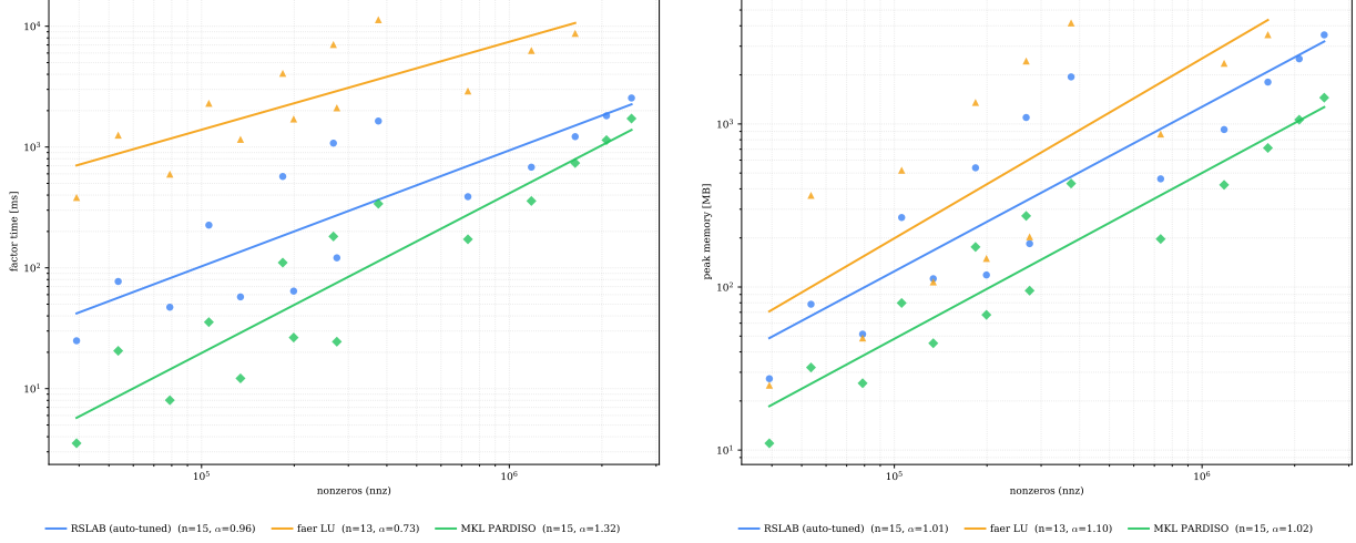
Figure 7: LU path (unsymmetric, PARDISO mtype 13): factor time (left) and peak memory (right) vs. problem size. On time RSLAB scales flatter than PARDISO ( \alpha \approx 0.96 vs. 1.32), closing the gap on large problems.
